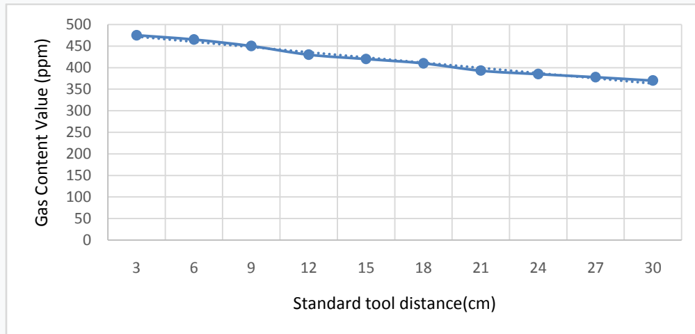
Figure 4. Graph of Standard tool distance vs Gas Content Value
