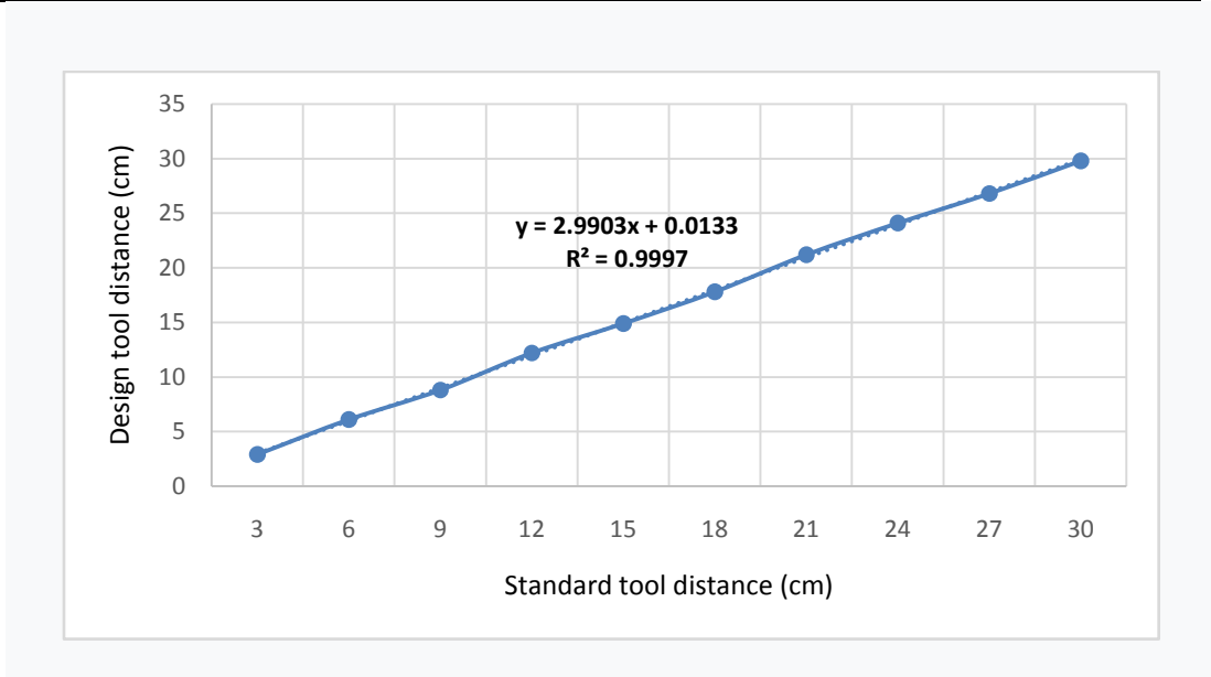
Figure 3. Graph of Standard tool distance vs Design tool distance
