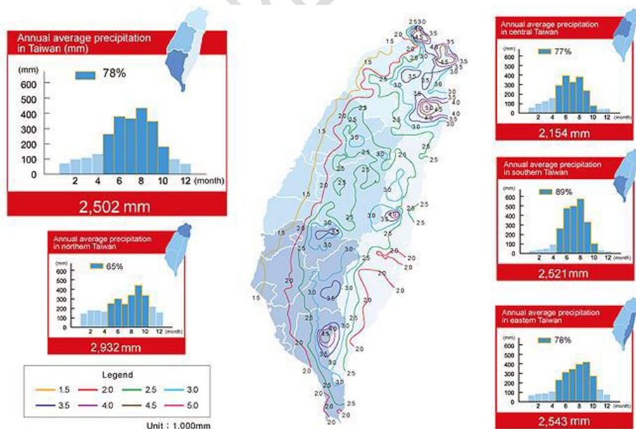
Figure 7. Isohyet Chart of Rainfall of Taiwan
