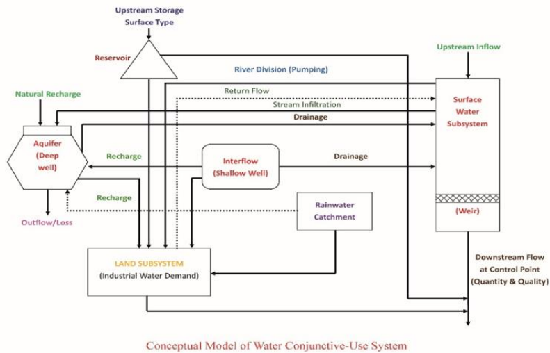
Fig.8 Conceptual Model of Water Conjunctive-Use System.
