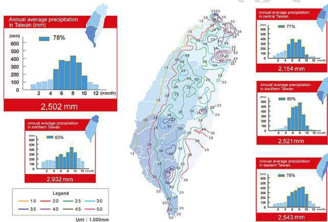
Figure 7. Isohyet Chart of Rainfall of Taiwan
