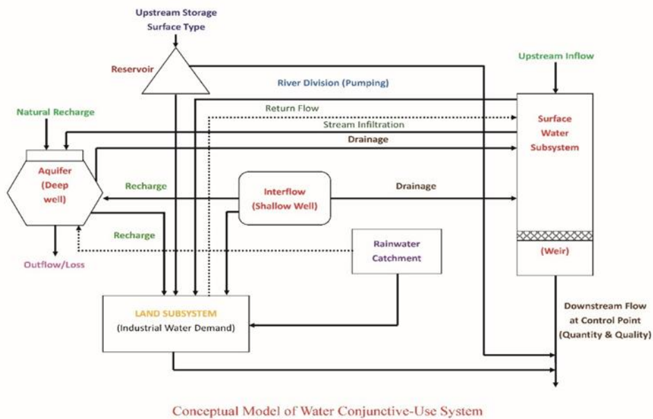
Fig.8 Conceptual Model of Water Conjunctive-Use System.
