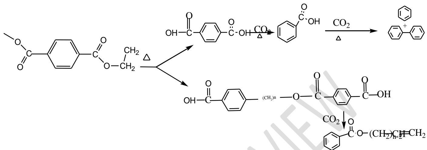
Figure 2: PET degradation
