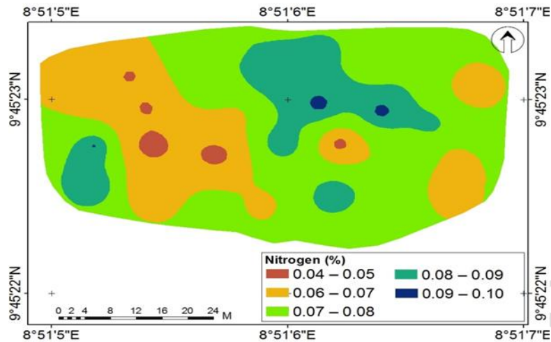
Fig. 5. Spatial distribution of N contents in the study area
