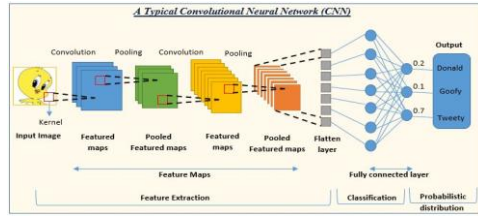
Fig.1 CNN Architecture
