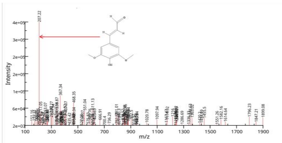
Fig 7 : Mass spectrum of 5-Hydroxy ferulate.
