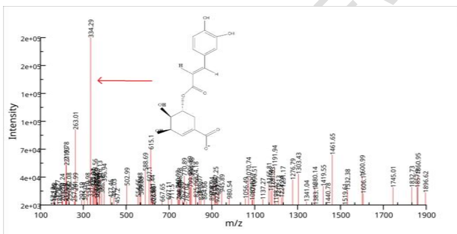
Fig 5: Mass spectrum of Caffeoyl shikimate
