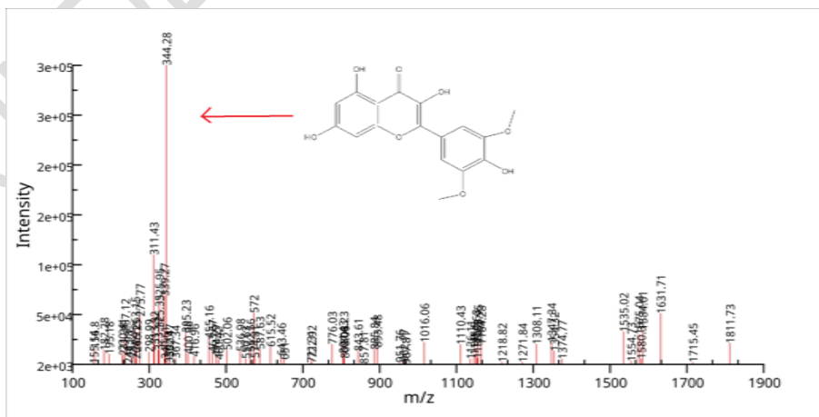
Fig 6: Mass spectrum of Syringetin
