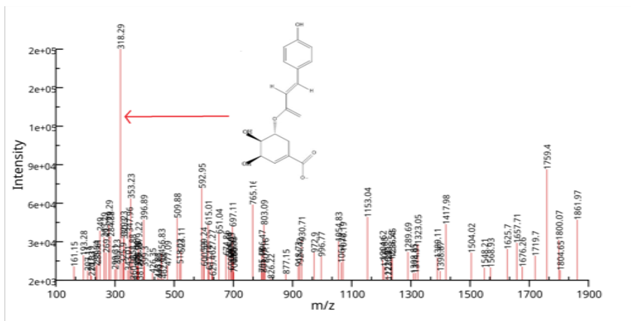
Fig 4 : Mass spectrum of p-Coumaroyl shikimate
