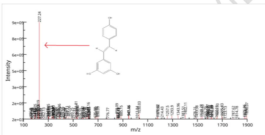
Fig 8 : Mass spectrum of Resveratrol
