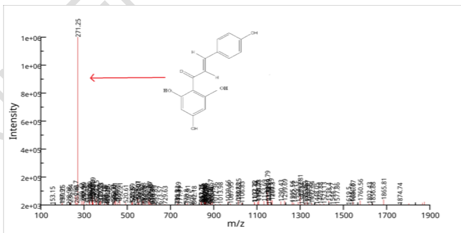
Fig 9: Mass spectrum of Naringenin chalcone.
