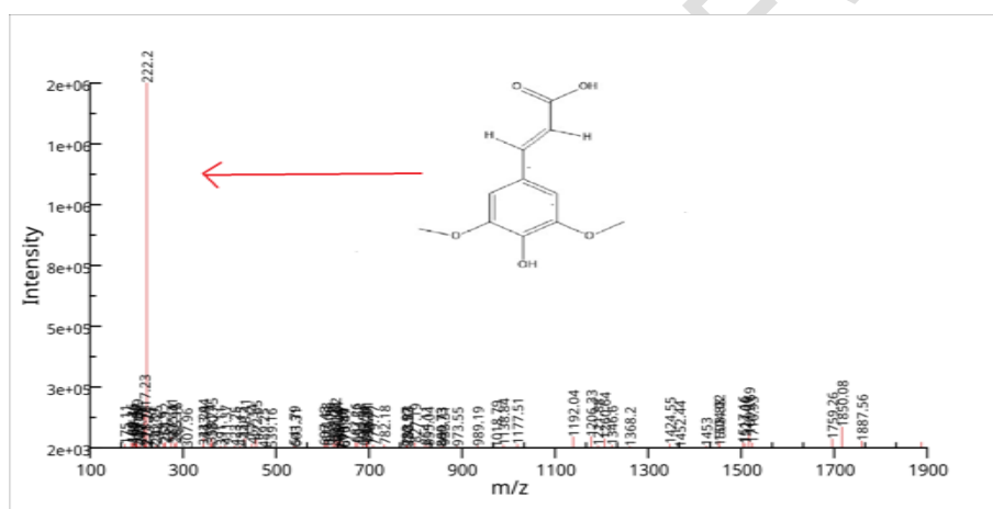
Fig 2: Mass spectrum of Sinapic acid
