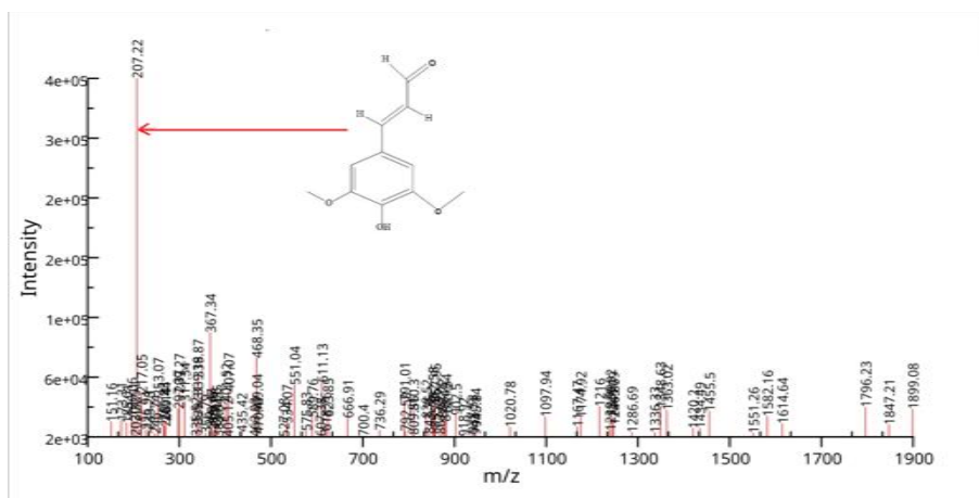
Fig 10 : Mass spectrum of Sinapaldehyde
