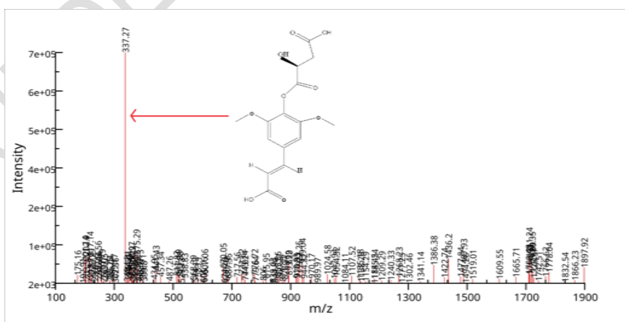
Fig 3: Mass spectrum of Sinapoyl malate
