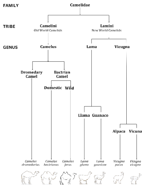
Fig. 1. Phylogeny of family Camelidae
