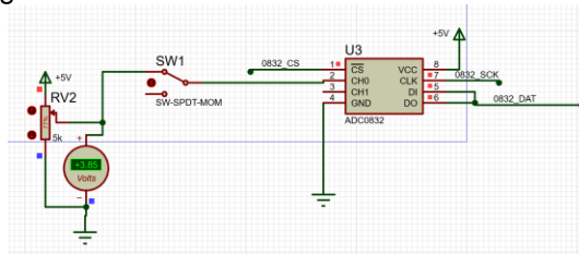
Fig. 15 Water level monitoring module and A/D conversion module circuit schematic diagram
