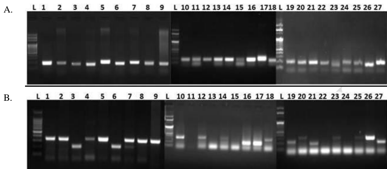
Fig. 2. Amplification pattern of A. RM8213 and B. RM10864 markers across all the genotypes.
