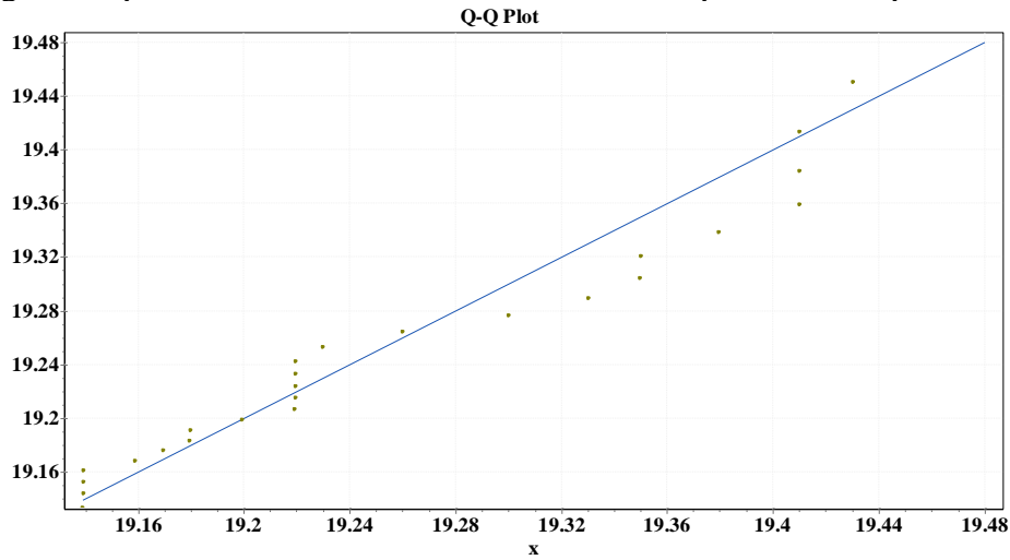
Fig.6: Q-Q plot for data set, and the fitted Burr CDF plots with empirical CDF
