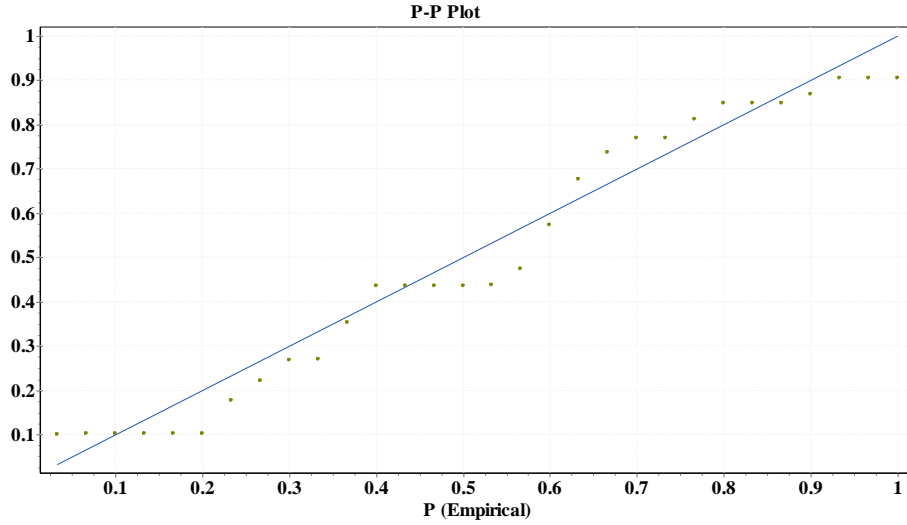
Fig.5: P-P plot for data set, and the fitted Burr CDF plots with empirical CDF
