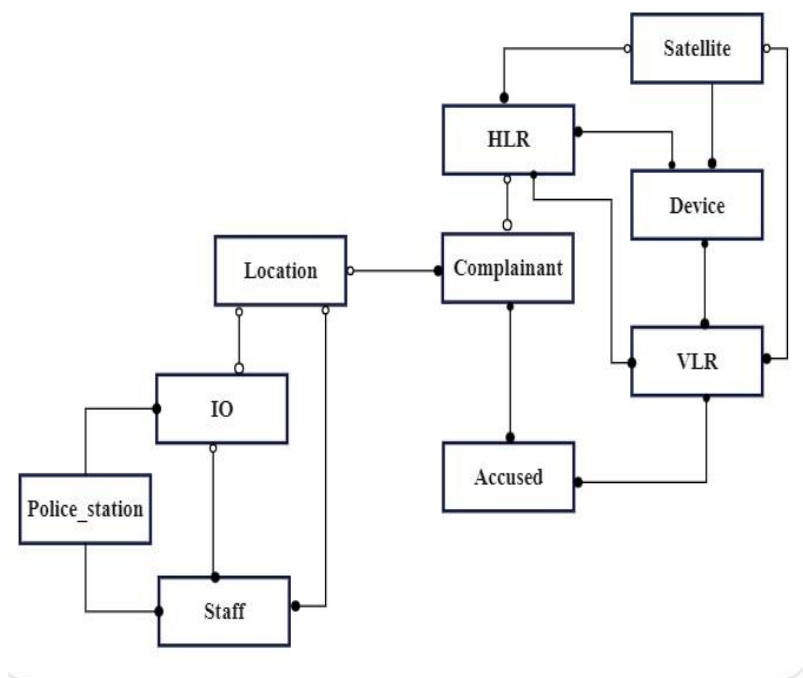
Figure 2. UML Model for Matching HLR with VLR
