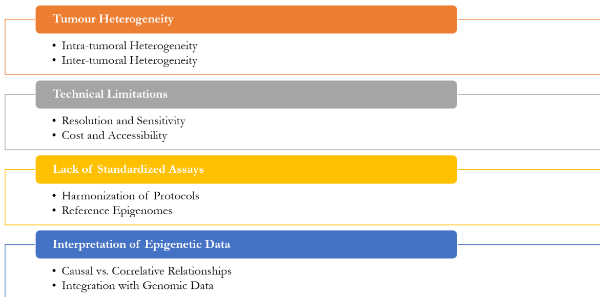
Figure 3: The challenges in epigenetic research lie in the diversity in cells that make the tumour, which can be intra-tumoral or intertumoral heterogeneity. Also, other challenges exist in the form of technical limitations – resolution and sensitivity as well as cost and accessibility; lack of standardised assay and limitations in the interpretation of epigenetic data also make up part of the challenges in epigenetic research in breast cancer.
