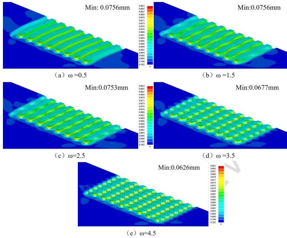
Fig 18 Sheet thickness distribution at different \omega
