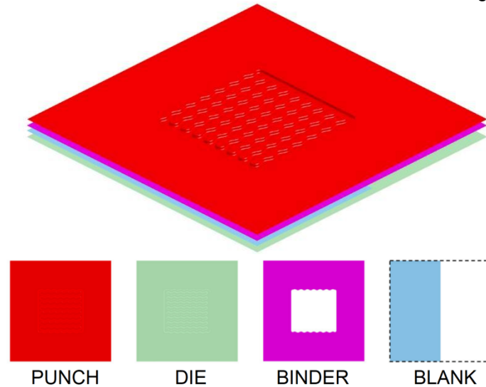
Fig 5 Diagram of tool positioning and parts layer
