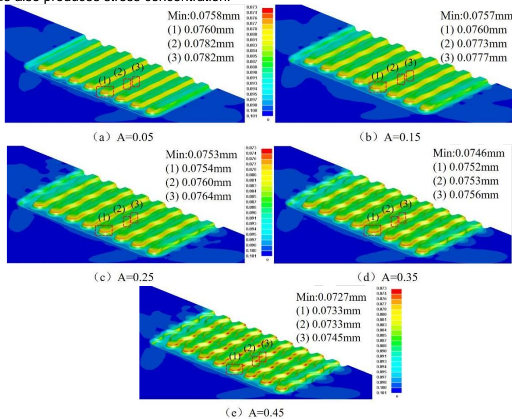
Fig 14 Sheet thickness distribution at different A
