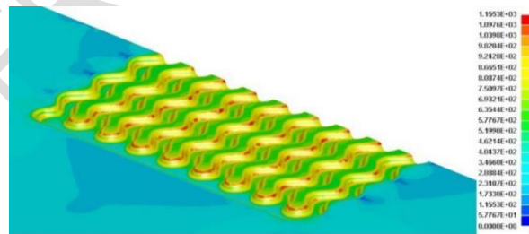
Fig 15 The Sheet Von Mises stress distribution at A=0.45
