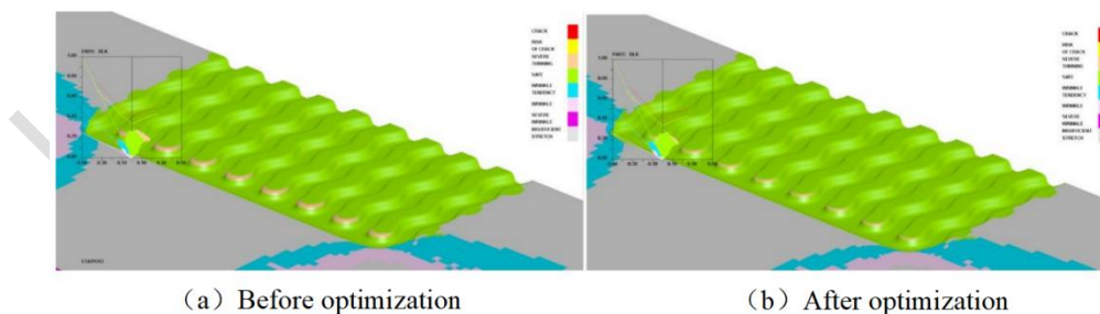
Fig 10 Sheetforming limit diagram before and after optimization
