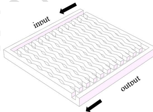
Fig 1 Bipolar plate flow field structure
