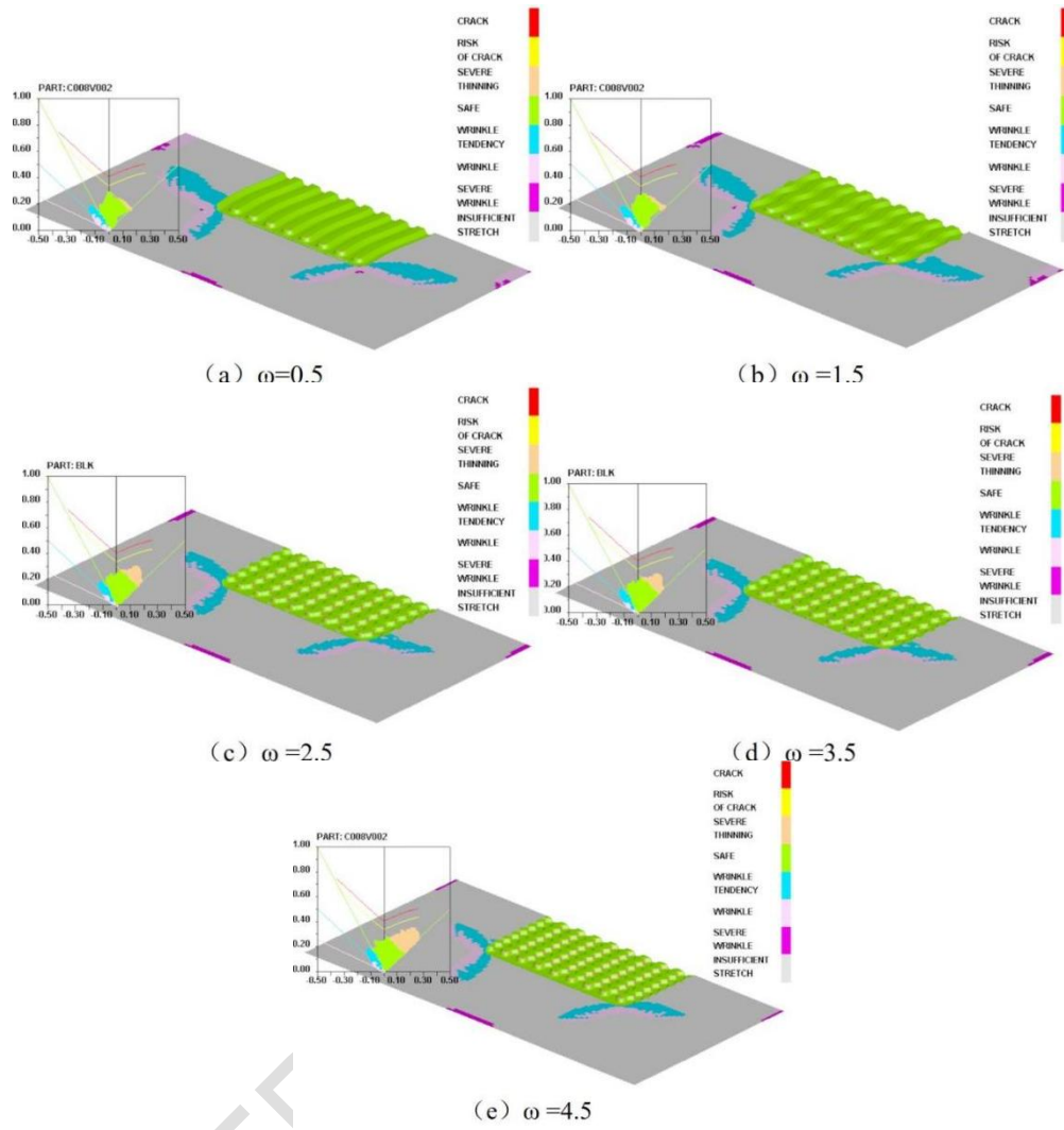
Fig 17 Sheetforming limit diagram at different \omega
