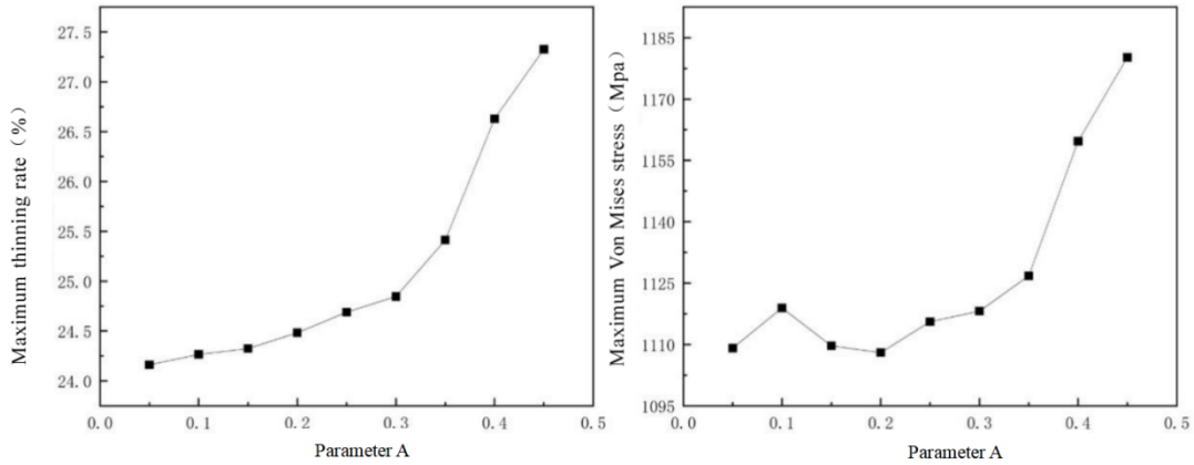
(a) Maximum thinning rate of sheet metal (b) Maximum V on Mises stress of sheet metal
