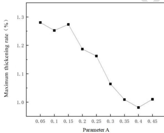
(c) maximum thickness increase of sheet metal
