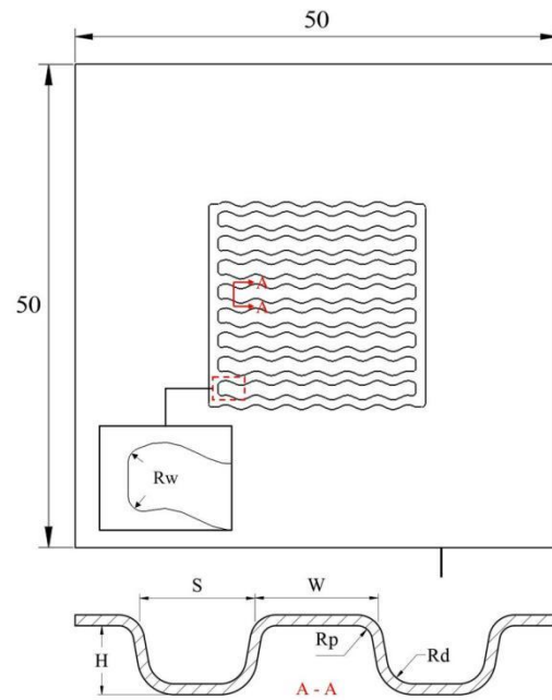
Fig 2 Simplified model of metal bipolar plate and size of flow channel
