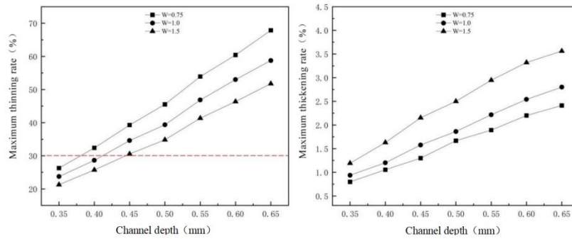
(b) S=1.0mm: maximum thinning rate and maximum thickening rate of sheet metal
