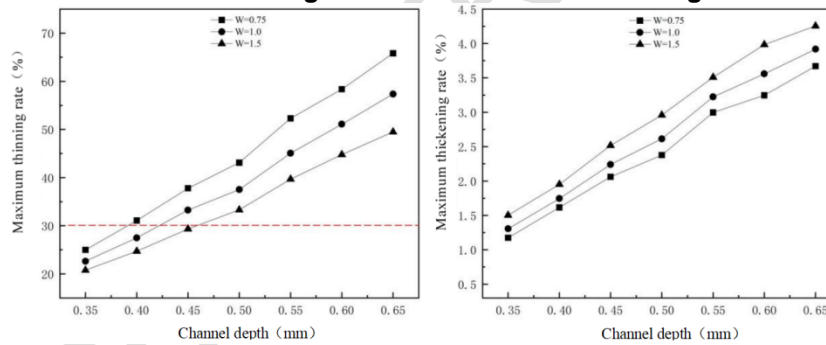
(c) S=1.5mm: maximum thinning rate and maximum thickening rate of sheet metal
