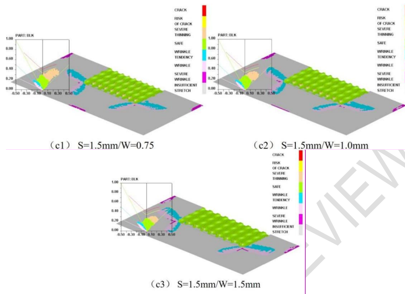
Fig5 Sheetforming limit diagram at different channelwidthand rib width combination
