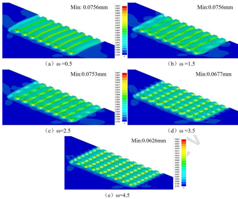
Fig 16 Sheet thickness distribution at different \omega
