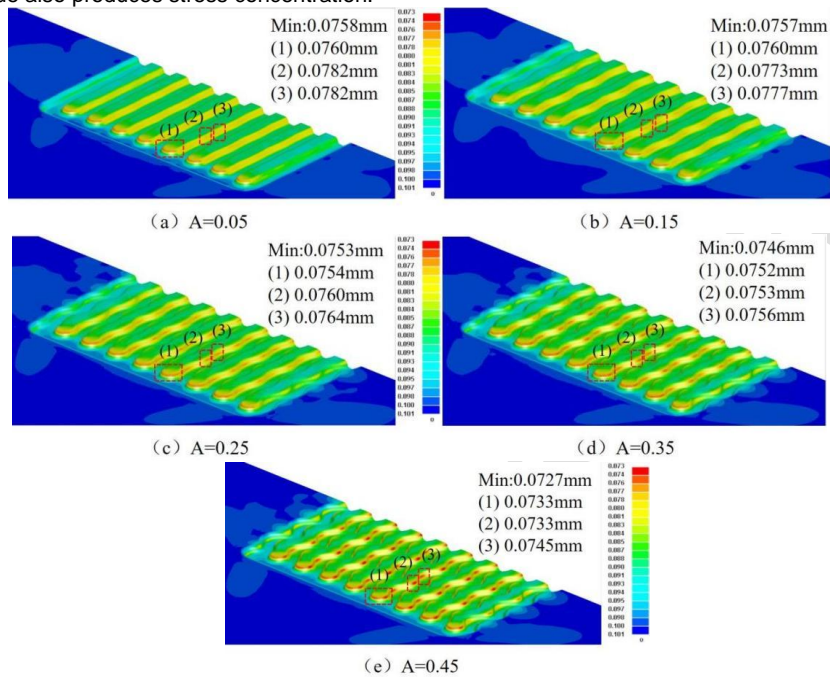
Fig 12 Sheet thickness distribution at different A
