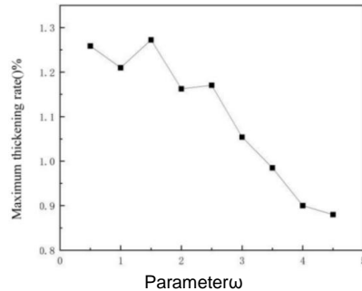
(c) maximum thickness increase of sheet metal
