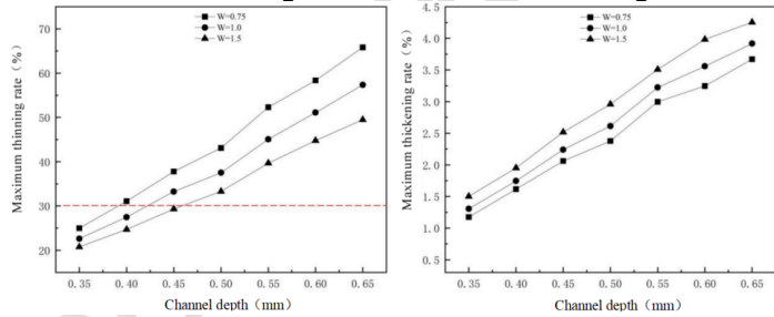
(c) S=1.5\text{mm} : maximum thinning rate and maximum thickening rate of sheet metal
