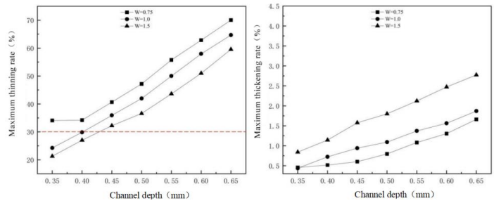
(a) S=0.5\text{mm} : maximum thinning rate and maximum thickening rate of sheet metal
