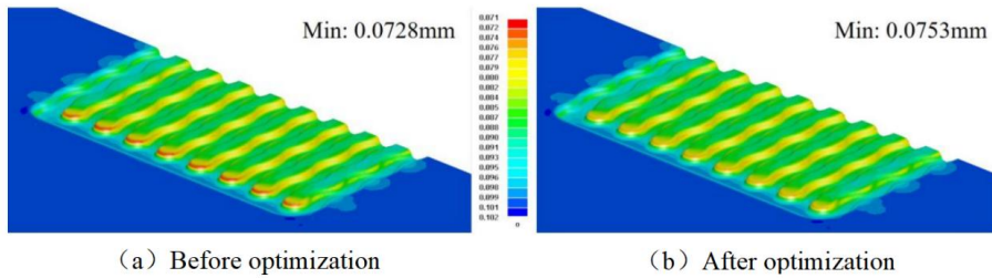
Fig 9 Sheetthickness distribution before and after optimization
