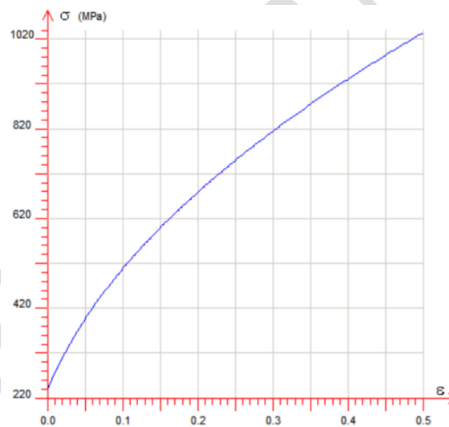
Fig 2 Stress-strain curve
