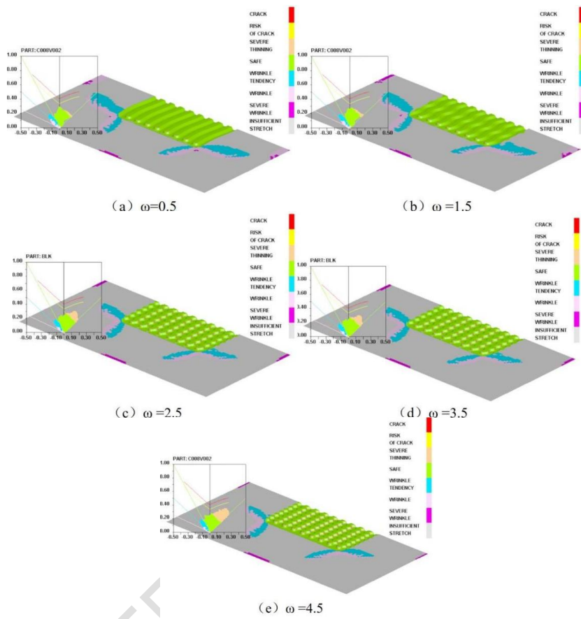
Fig 15 Sheetforming limit diagram at different \omega
