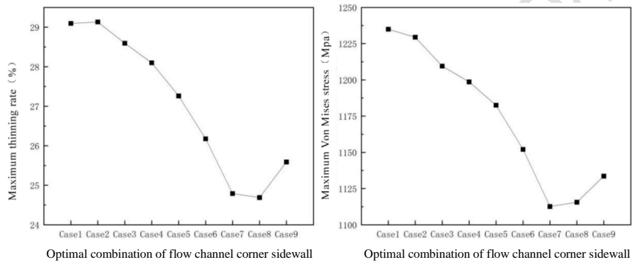
Fig 10 Simulation result at different \Delta H
