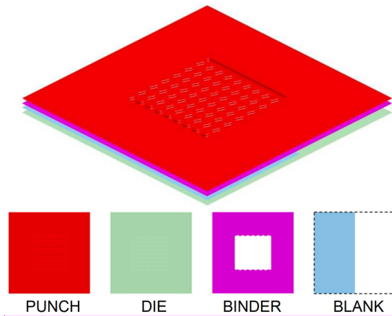
Fig 3 Diagram of tool positioning and parts layer
