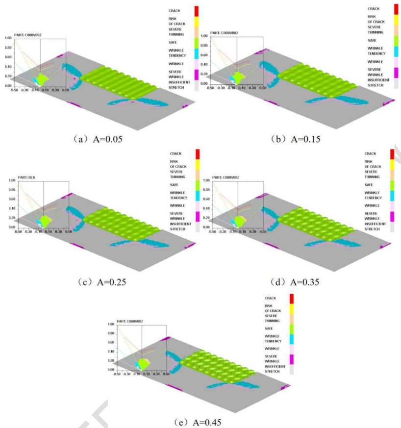
Fig 11 Sheetforming limit diagram at different A
