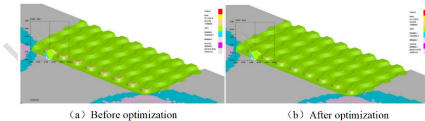
Fig 8 Sheetforming limit diagram before and after optimization
