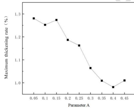
(c) maximum thickness increase of sheet metal
