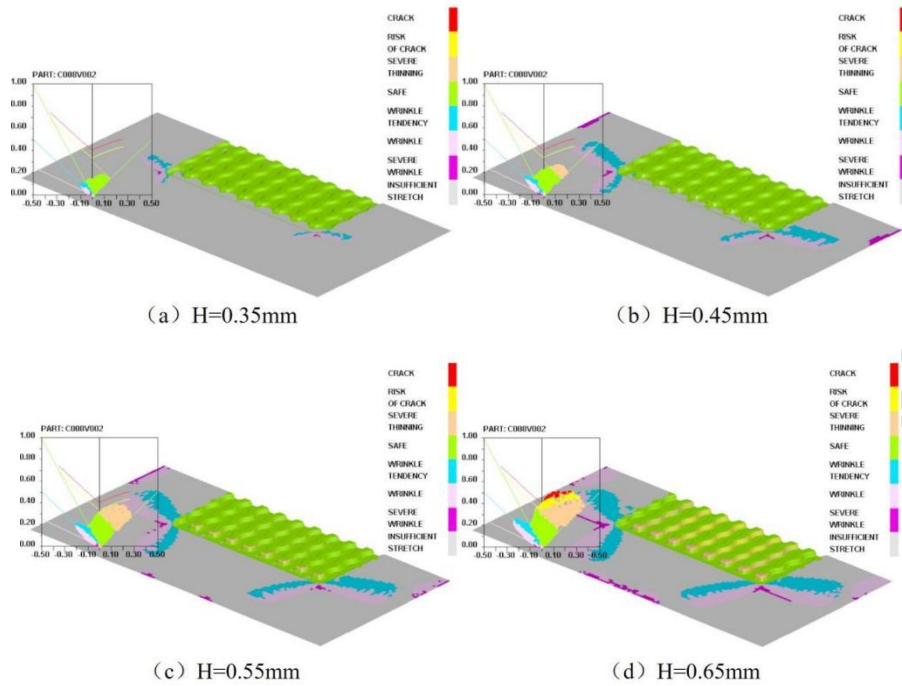
Fig4 Sheet forming limit diagram at different forming depths
