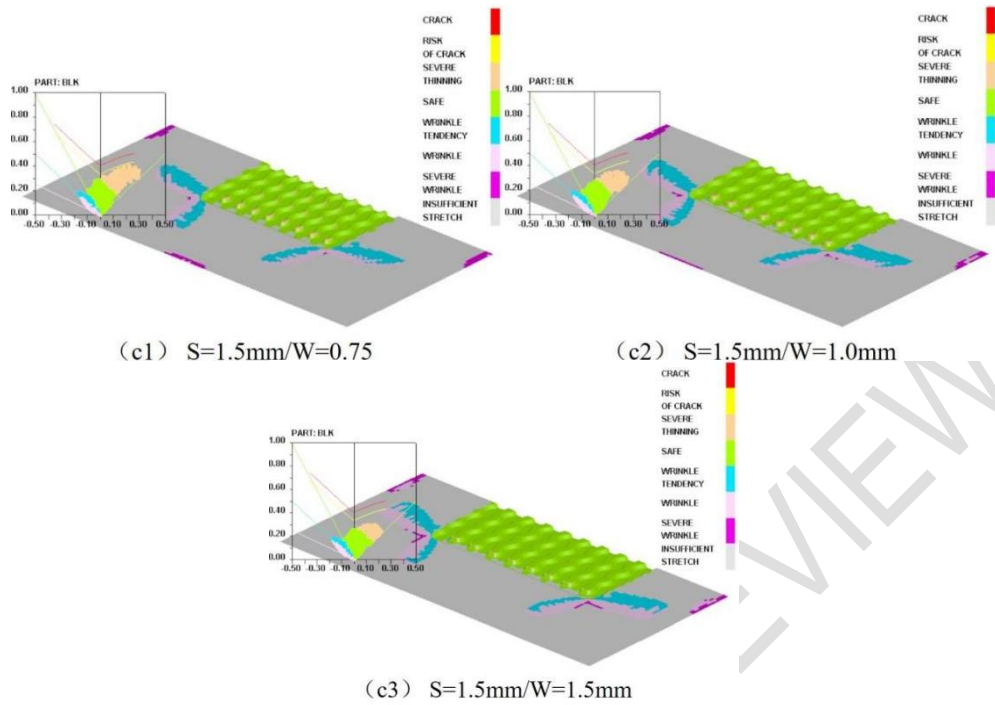
Fig5 Sheetforming limit diagram at different channelwidth and rib width combination
