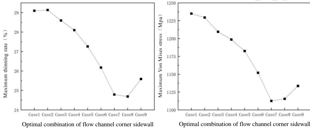
Fig 10 Simulation result at different \Delta H
