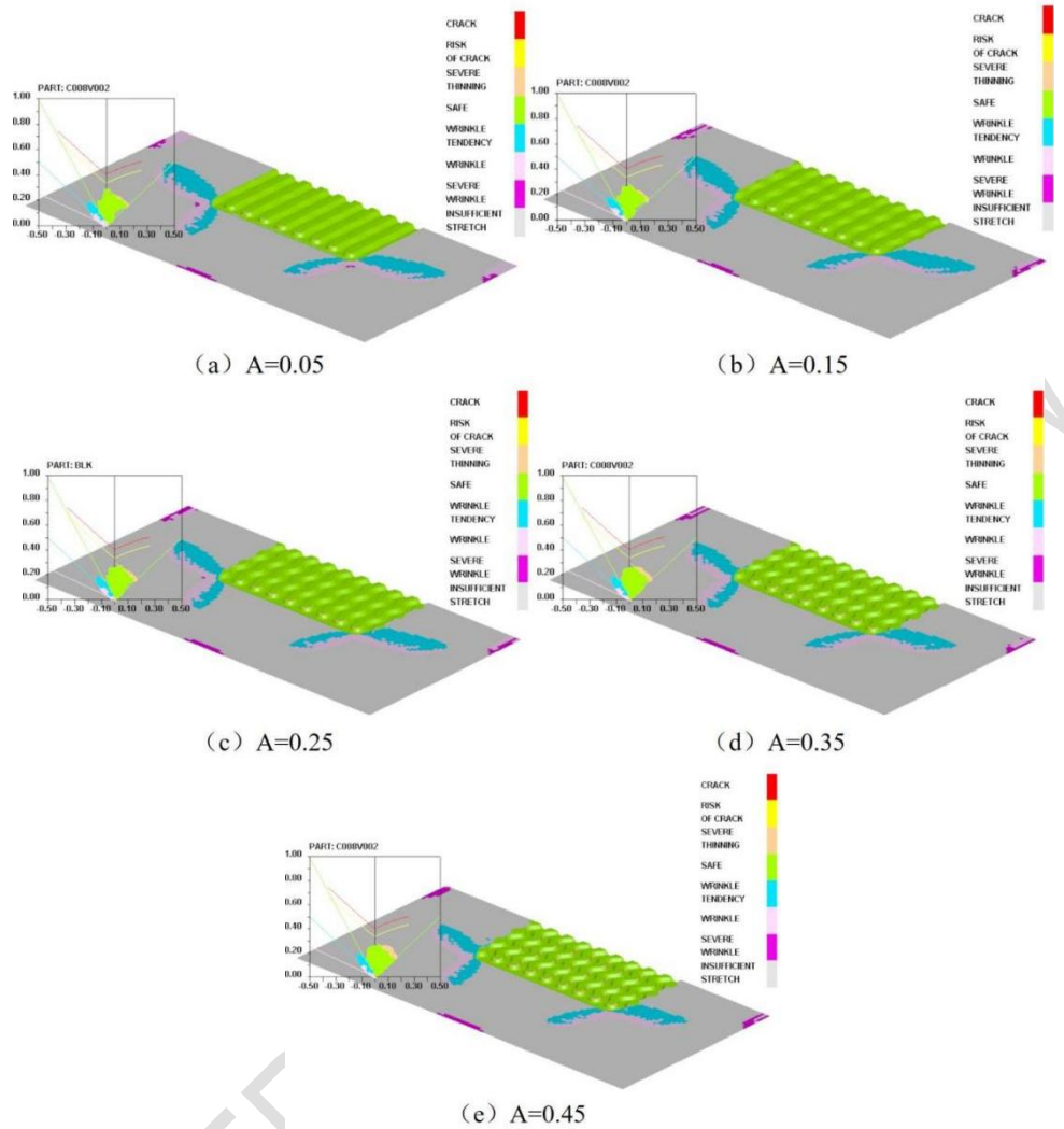
Fig 11 Sheetforming limit diagram at different A
