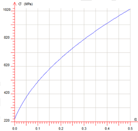
Fig 2 Stress-strain curve
