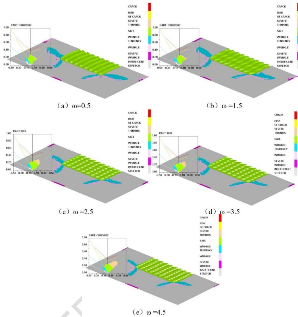
Fig 15 Sheetforming limit diagram at different \omega
