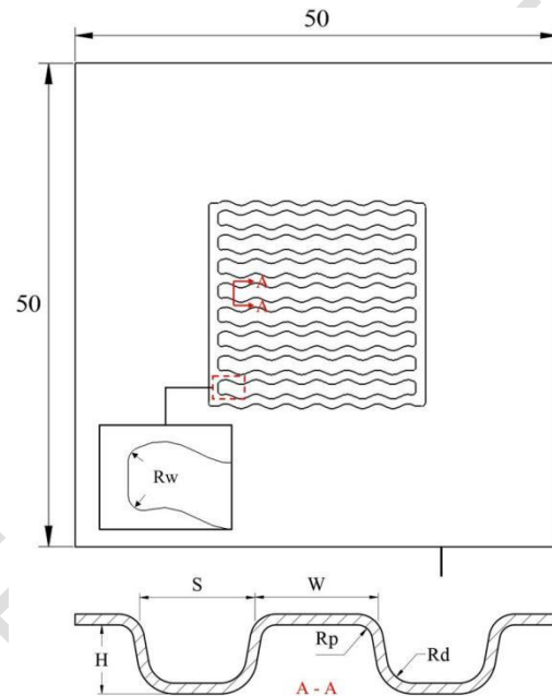
Fig 1 Simplified model of metal bipolar plate and size of flow channel
