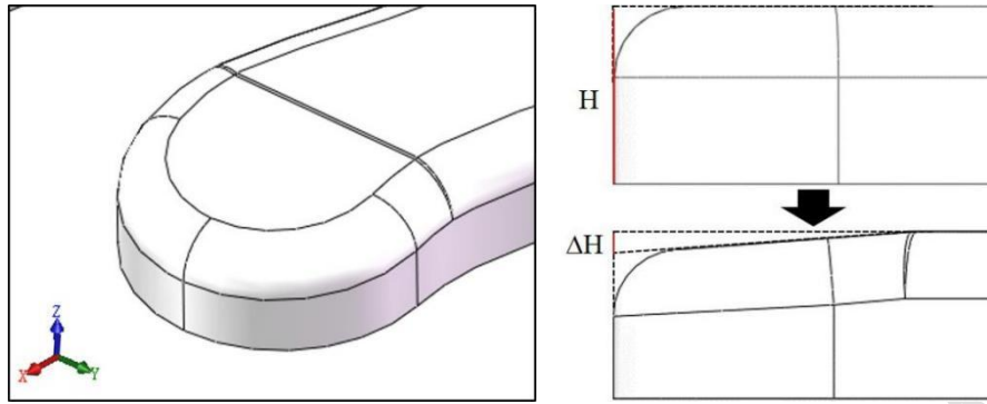
Fig 7 Rib height gradient structure
