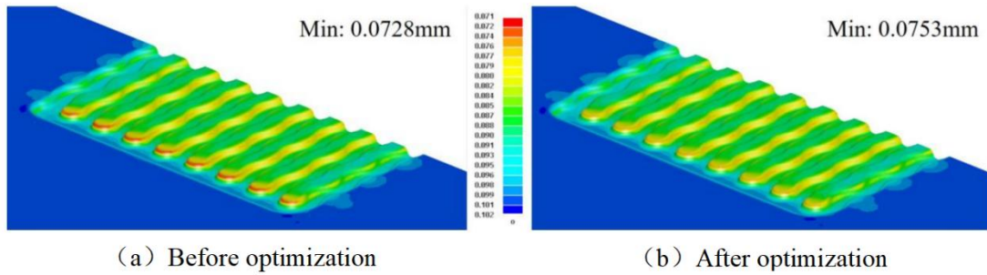
Fig 9 Sheetthickness distribution before and after optimization
