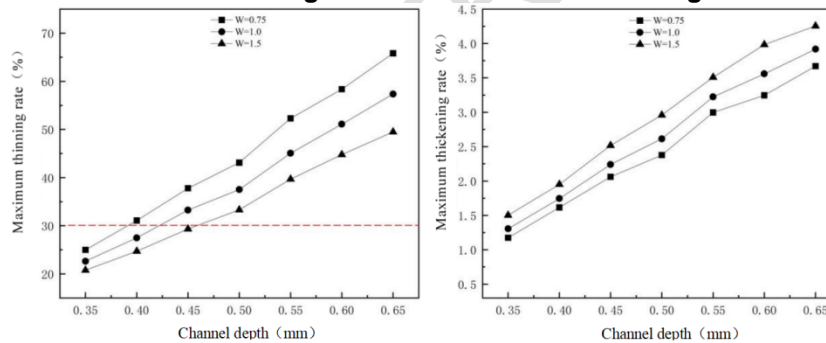
(c) S=1.5mm: maximum thinning rate and maximum thickening rate of sheet metal
