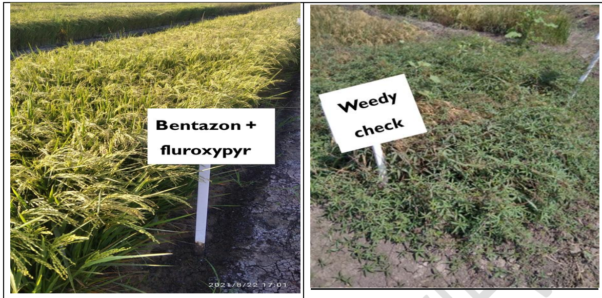
Fig. 1: Rice growth in plots treated with bentazon + fluroxypyr as compared to weedy check plots under study conditions.
