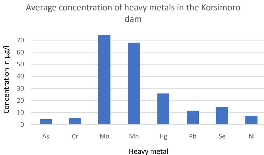
Figure 2: Average concentrations of metallic trace elements in the Korsimoro dam
