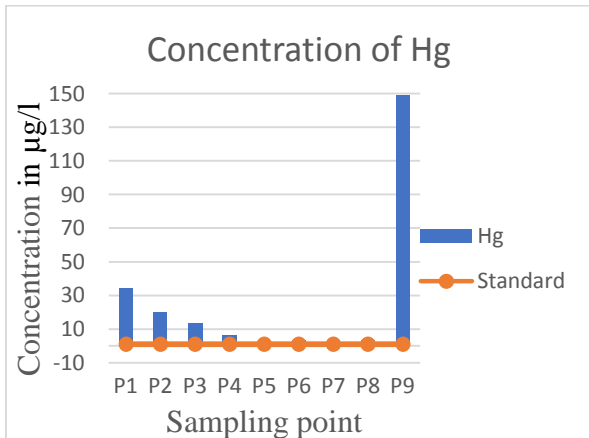
Figure 7: Mercury concentration by sampling point
