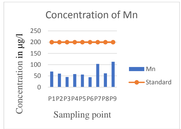
Figure 6: Manganese concentration by sampling point
