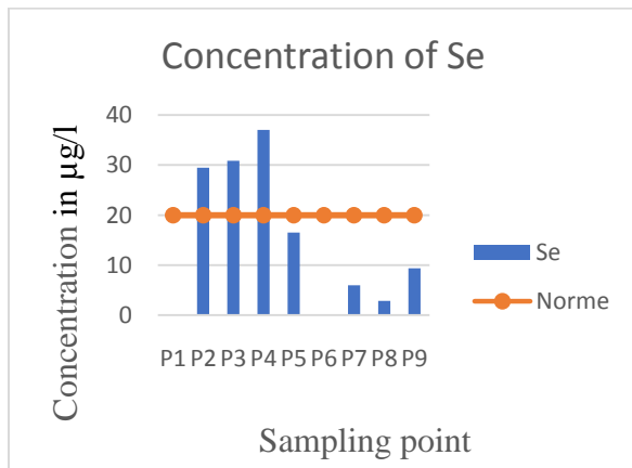
Figure 9 :Selenium concentration by sampling point
