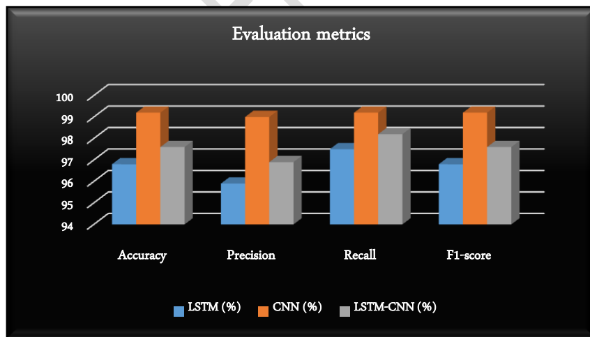
Figure 10: Evaluation metrics
