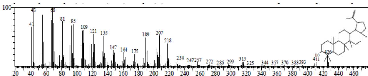
Fig. 7. Mass spectrum of Lupeol (RT: 26.535, Area % = 1.97)
