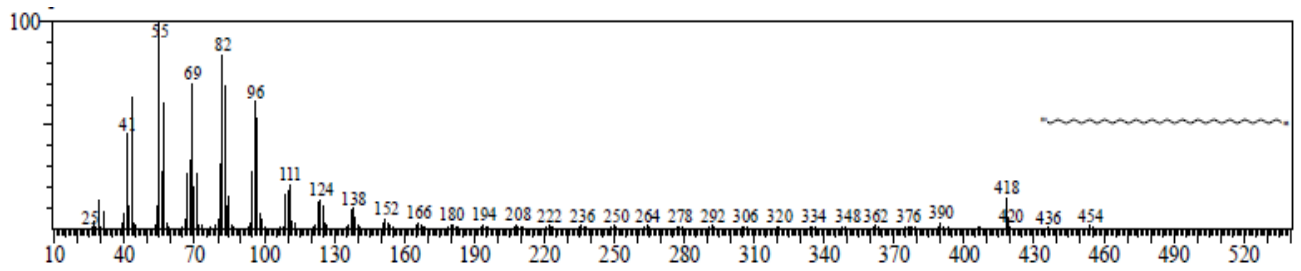
Fig. 10. Mass spectrum of 1,30-Triacontanediol (RT: 30.234, Area % = 34.47)
