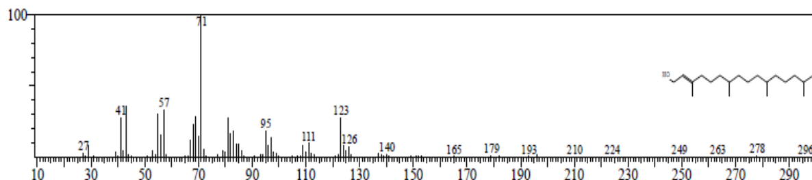
Fig. 5. Mass spectrum of Phytol (RT: 20.262, Area % = 1.36)
