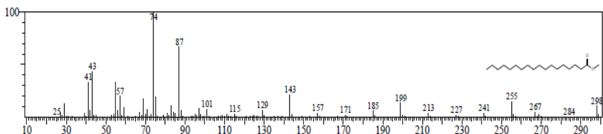
Fig. 6. Mass spectrum of Methyl stearate (RT: 20.382, Area % = 2.08)
