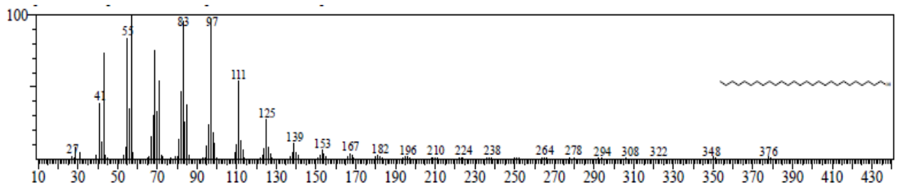
Fig. 11. Mass spectrum of 1-Heptacosanol (RT: 30.348, Area % = 1.89)
