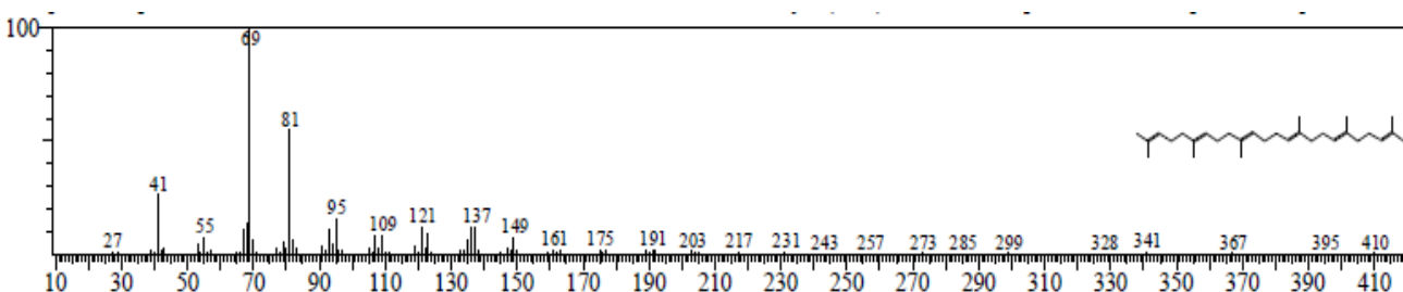
Fig. 9. Mass spectrum of Squalene (RT: 29.351, Area % = 32.75)
