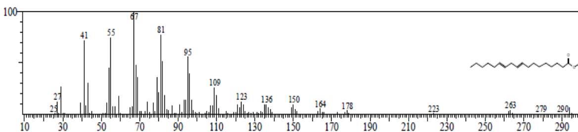
Fig. 3. Mass spectrum of Hexadecanoic acid, methyl ester (RT: 17.498, Area % = 3.82)
