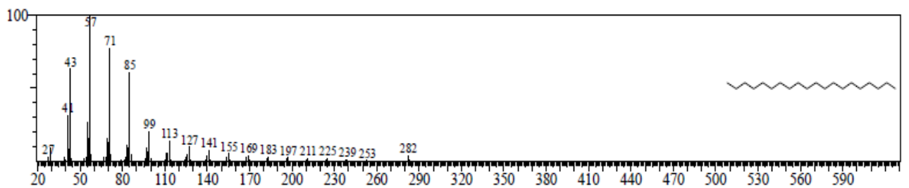
Fig. 12. Mass spectrum of Eicosane (RT: 30.635, Area % = 0.88)
