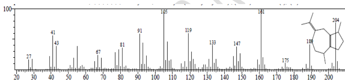
Fig. 2. Mass spectrum of Beta-Guaiene (RT: 14.684, Area % = 0.85)
