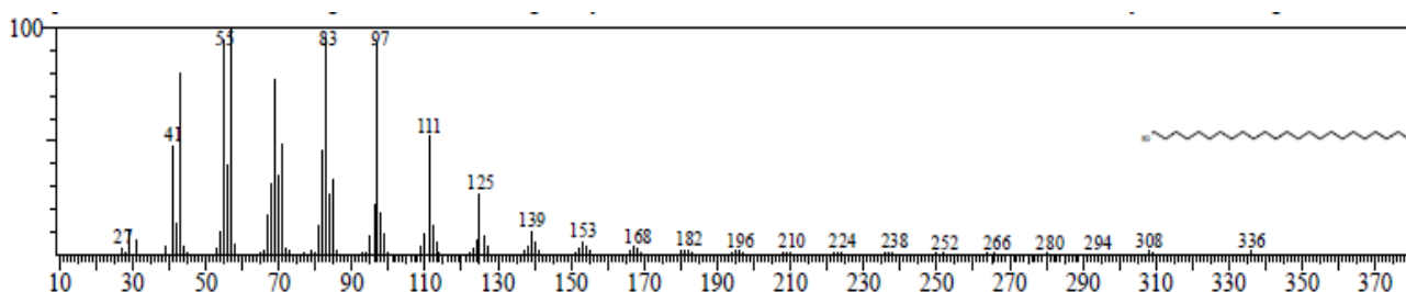
Fig. 8. Mass spectrum of n-Tetracosanol-1 (RT: 27.437, Area % = 17.34)
