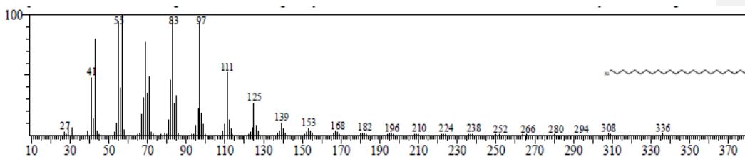
Figure8: Mass spectrum of n-Tetracosanol-1 (RT: 27.437, Area % = 17.34) from D. zibethinus seeds
