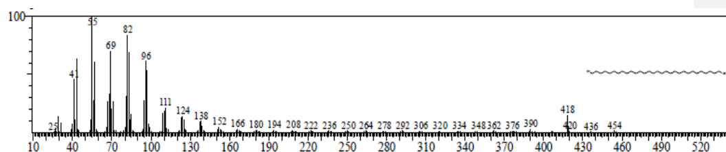
Figure10: Mass spectrum of 1,30-Triacontanediol (RT: 30.234, Area % = 34.47) from D. zibethinus seeds
