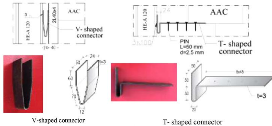
Fig.2. V-connector Fig.3. T type connector
