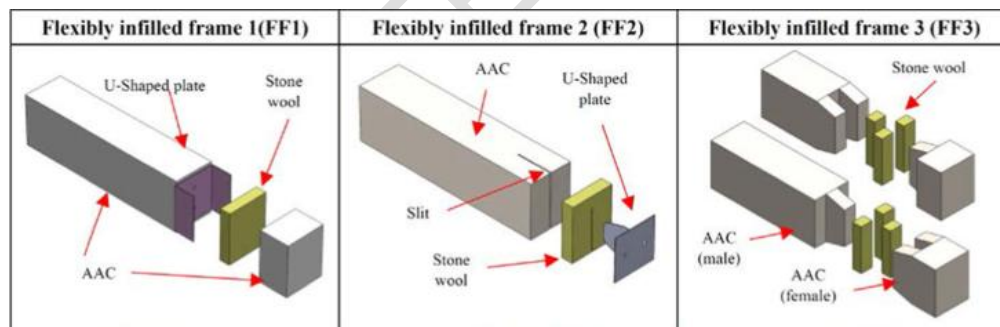
Fig. 1. Flexible connectors
