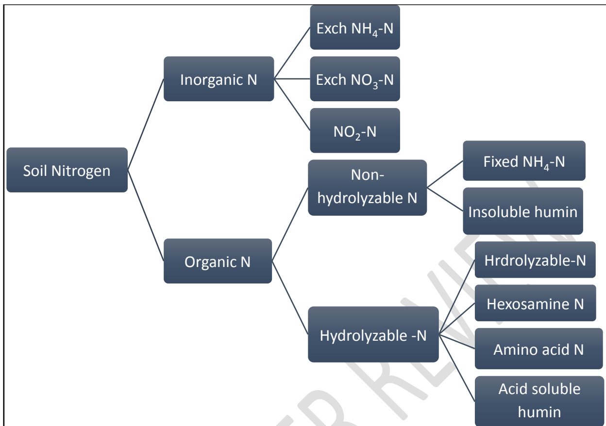
Fig 1. Flow diagram of different forms of soil N
