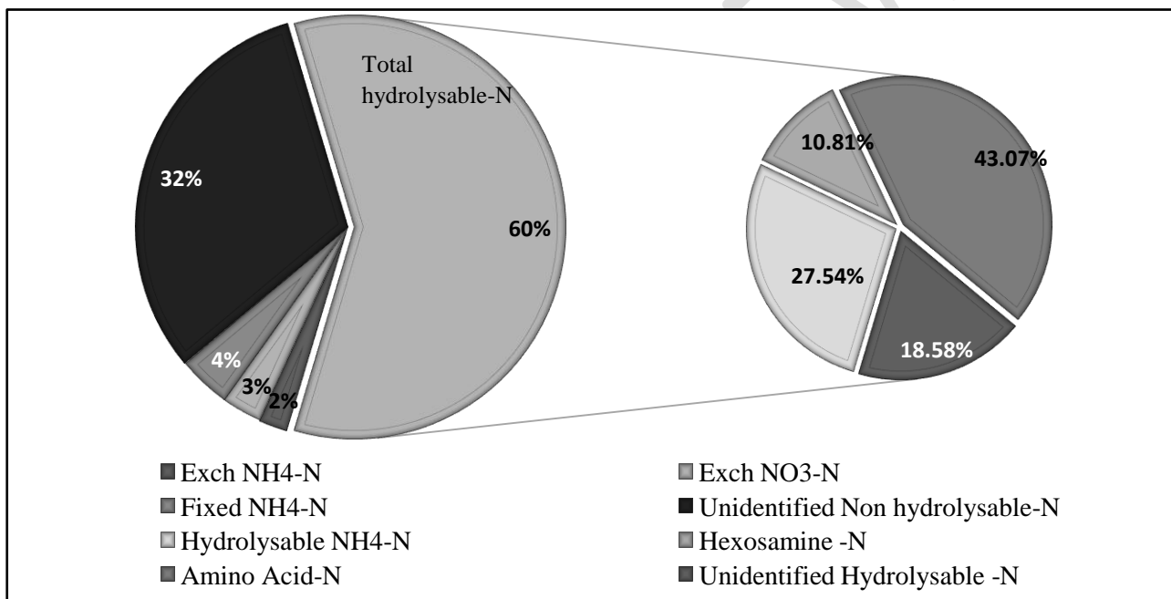
Fig 2. General contribution of nitrogen forms in arable land use system
