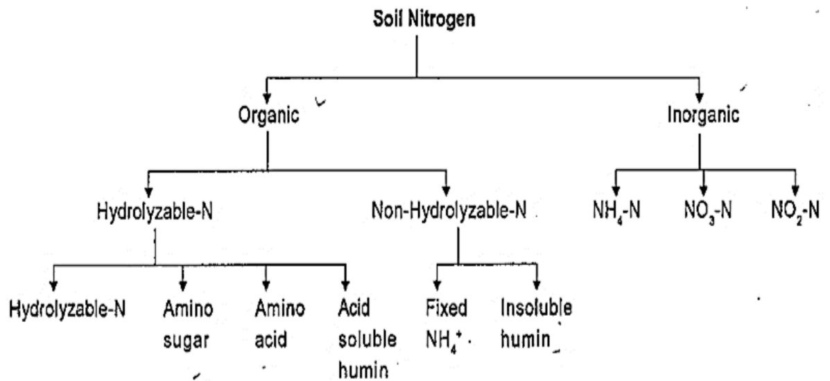
Fig 1. Flow diagram of different forms of soil N (Source: Tusneem and Patrick, 1971)
