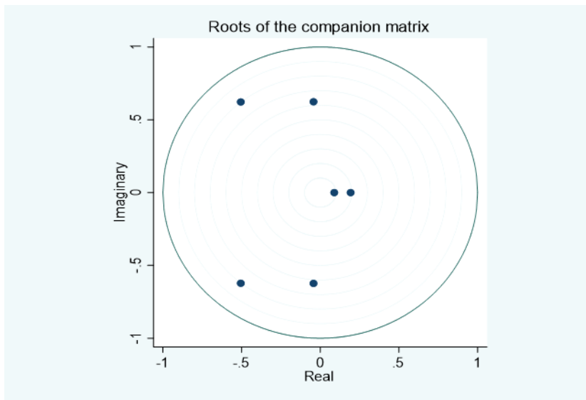
Fig. 1. Model AR root test results
