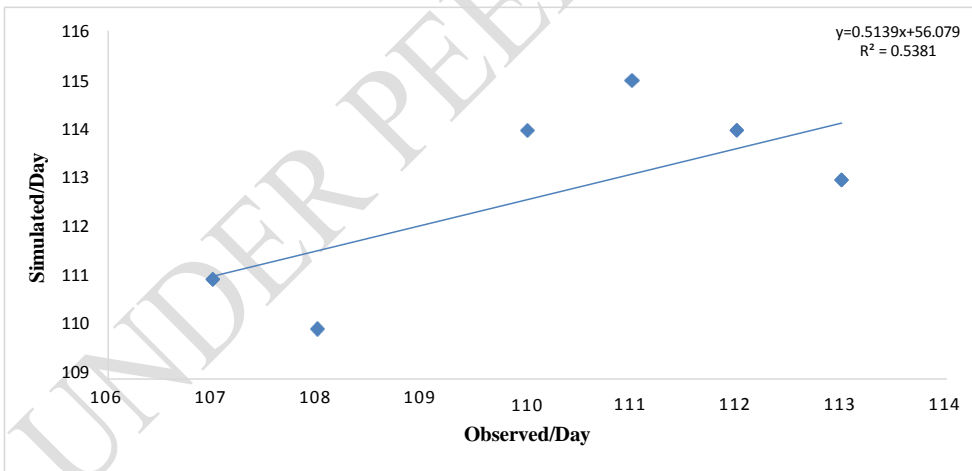
Fig:5 Observed and simulated values of physiological maturity day.
