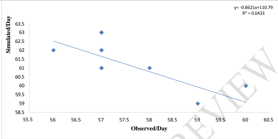
Fig:4 Observed and simulated anthesis days.
