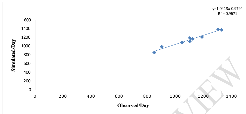
Fig.3 Observed and simulated grain yield (kg/h).
