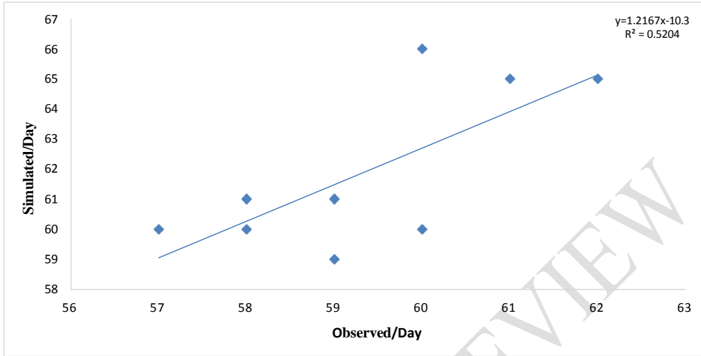
Fig:1 Simulated and observed anthesis days.
