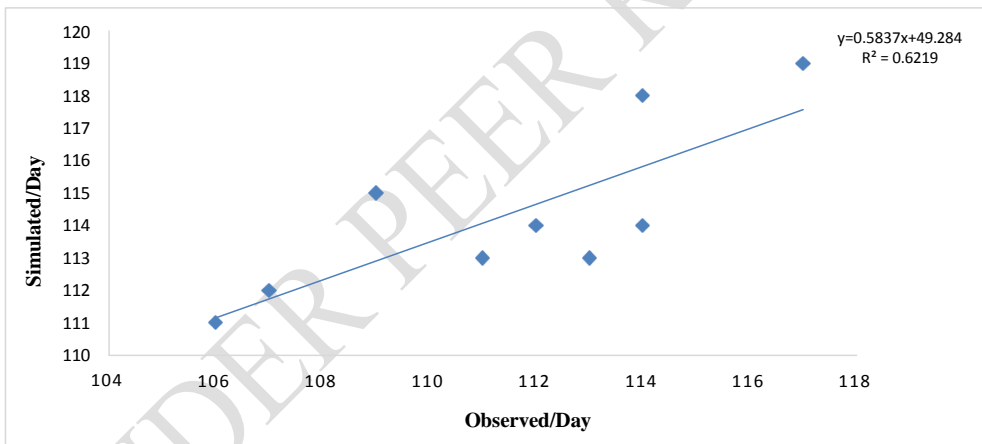
Fig:2 Observed and simulated physiological maturity days.
