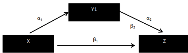
Fig. 1. Path Analysis Model
