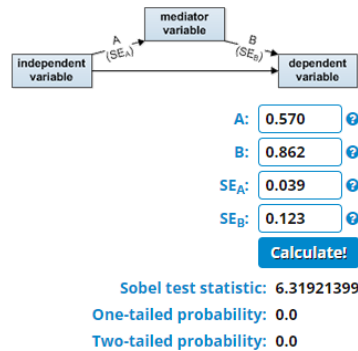
Fig. 2. Sobel test results
