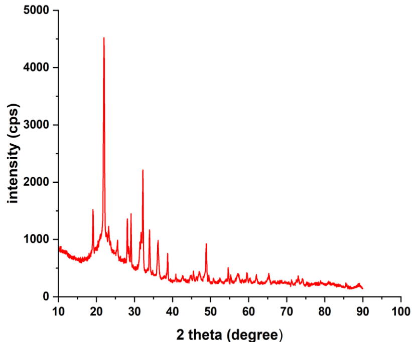
Fig 5. X-ray spectra showing crystalline nature of Silica nanoparticles
