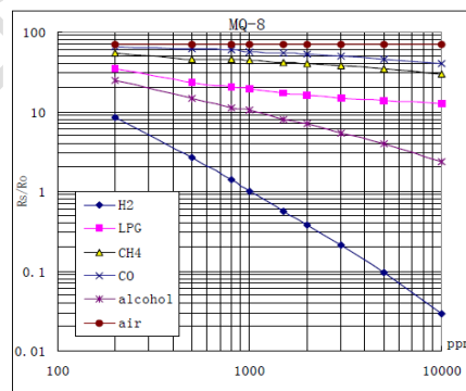
Figure 4 : MQ-8 sensitivity to different gases
