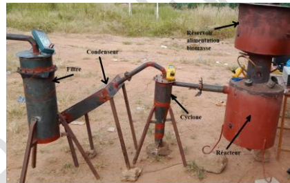
Figure 1 : Experimental setup
