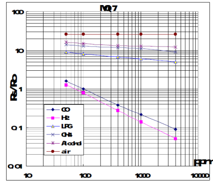
Figure 5 : MQ-7 sensitivity characteristics
