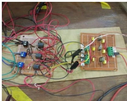
Figure 12 : Treatment and power supply boards
