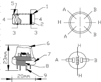
Figure 3 :MQ gas sensors structure
