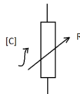
Figure 2 : Electrical model of a MQ gas sensor
