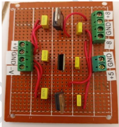
Figure 11 : Main power module
