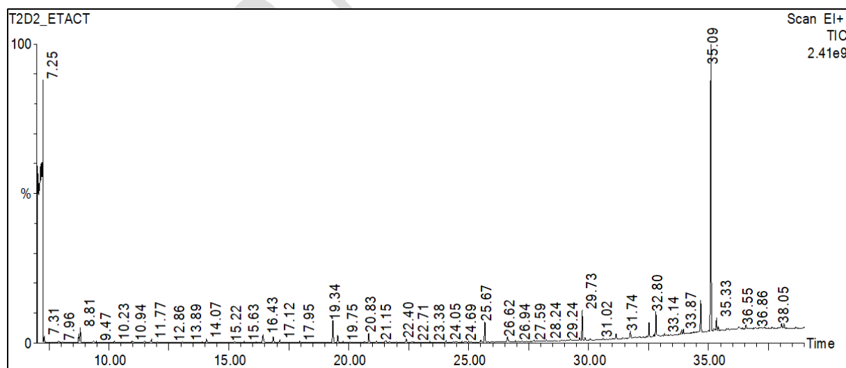
Figure 3: GC-MS chromatogram of the ethyl acetate extract of secondary metabolite produced by T. longibrachiatum L2D2 reveals the presence of volatile compounds.
