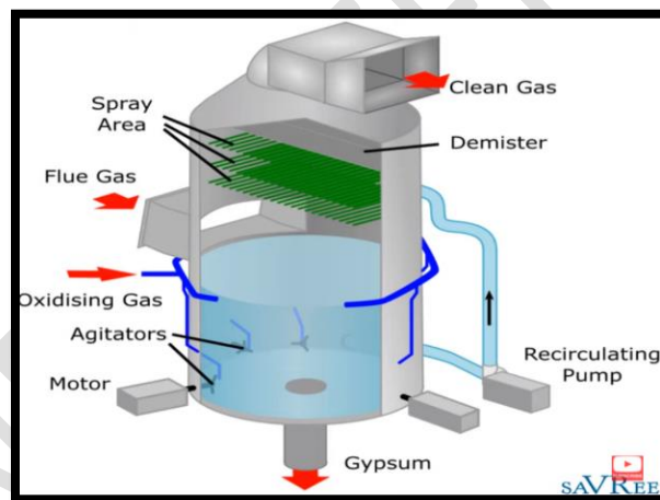
Fig. 1: Flue gas desulphurization equipment
