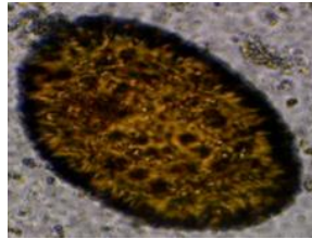
Plate 2 P. westermani
