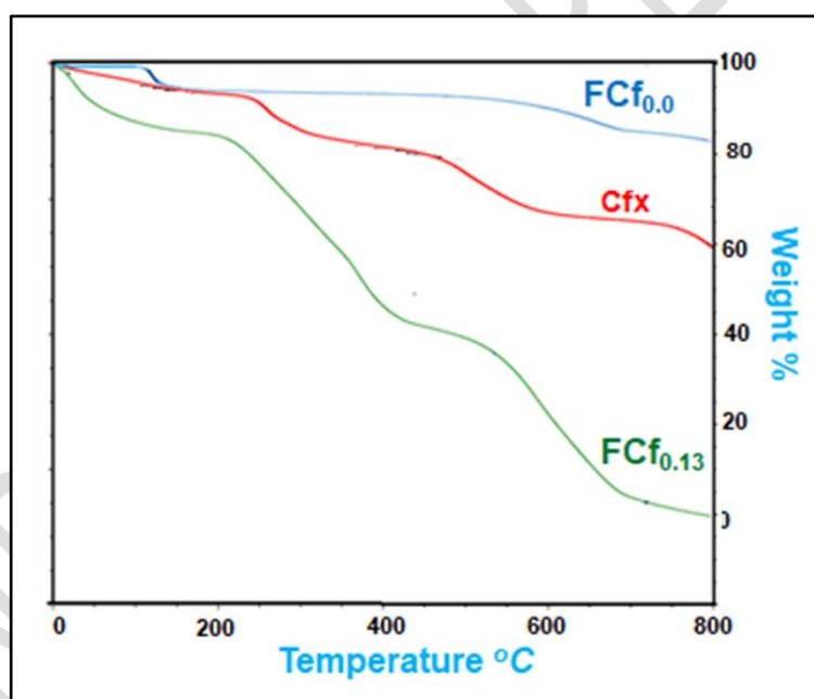
Fig.4. Thermo-gravimetric analysis curves of (a) Plain KCl crosslinked KC film FCf 0.0 , (b) drug Ciprofloxacin and (c) Composite film FCf 0.13 (Defence Institute of Advance Technology, Pune).
