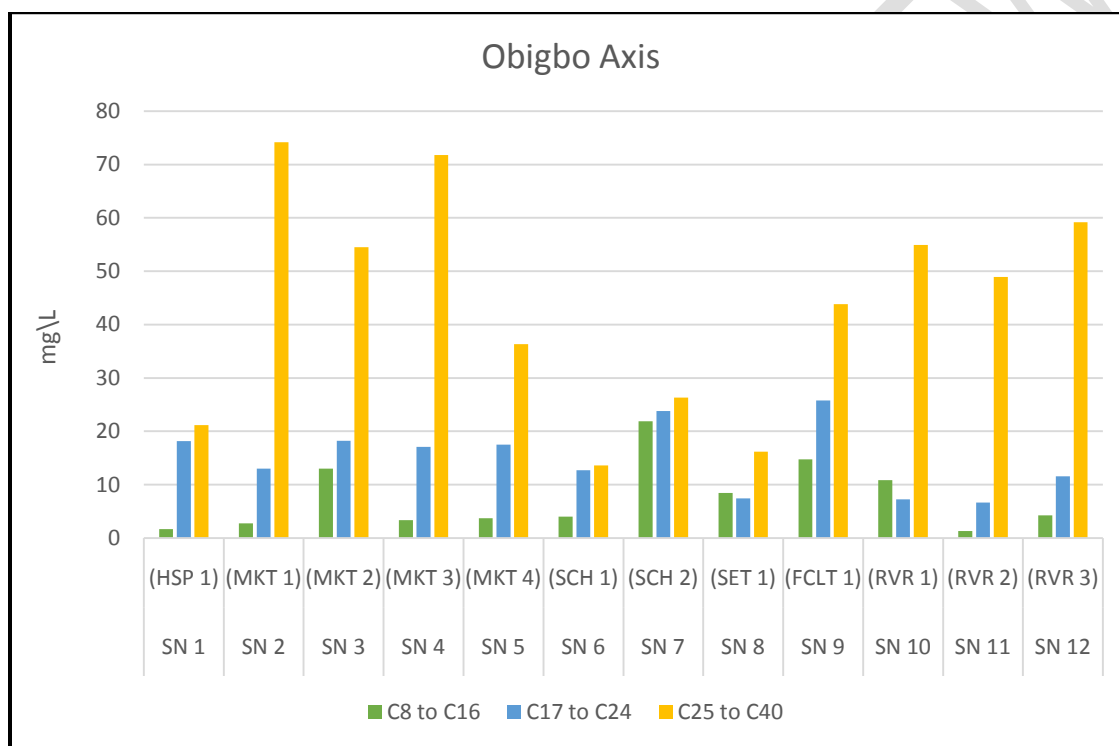
Figure 6a: Aliphatic Hydrocarbons Distribution Chart for Obigbo Study Axis
