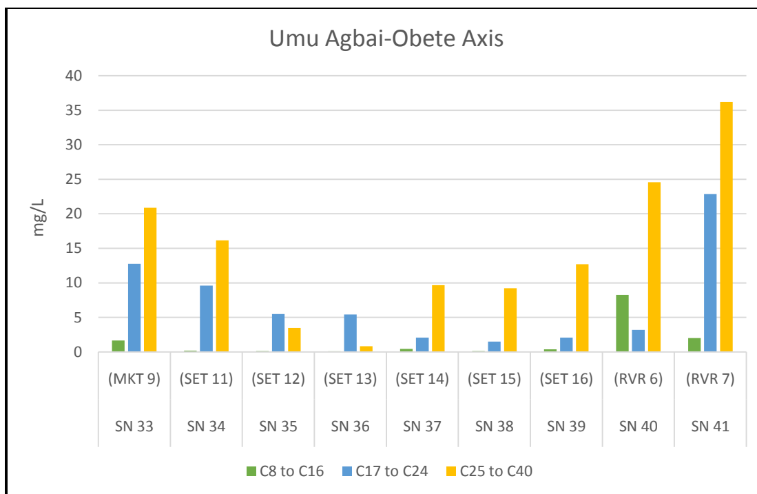
Figure 6e: Aliphatic Hydrocarbons Distribution Chart for Umu Agbai-Obete Study Axis
