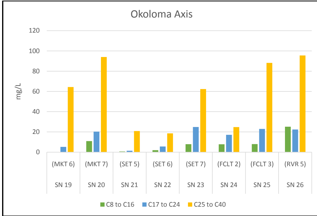
Figure 6c: Aliphatic Hydrocarbons Distribution Chart for Okoloma Study Axis
