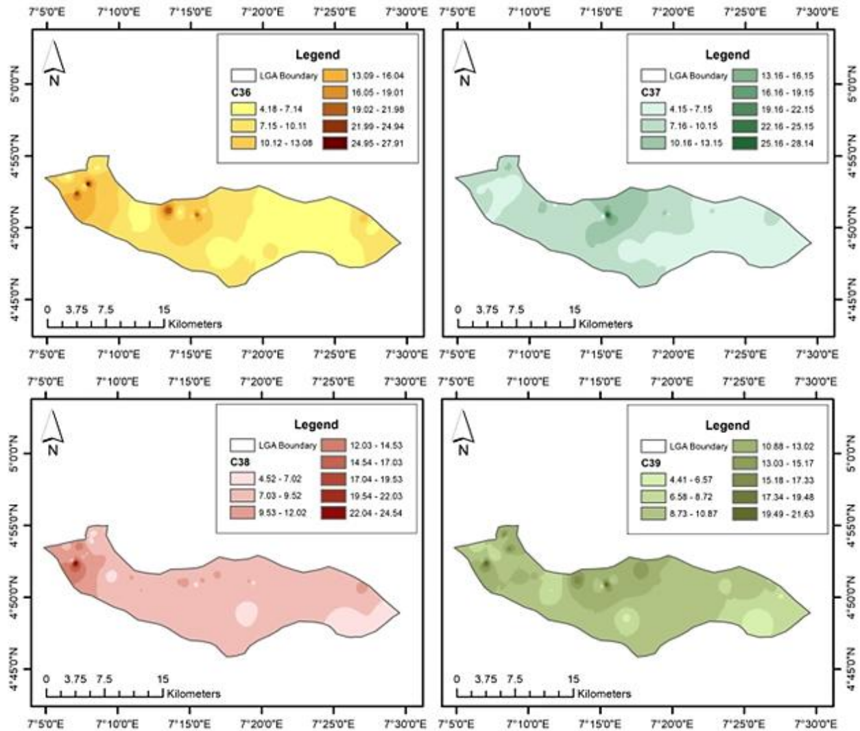
Figure9g: Spatial variations of C 36 to C 39 Aliphatic Hydrocarbon contents across the Study Area
