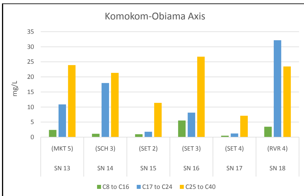
Figure 6b: Aliphatic Hydrocarbons Distribution Chart for Komokom-Obiama Study Axis
