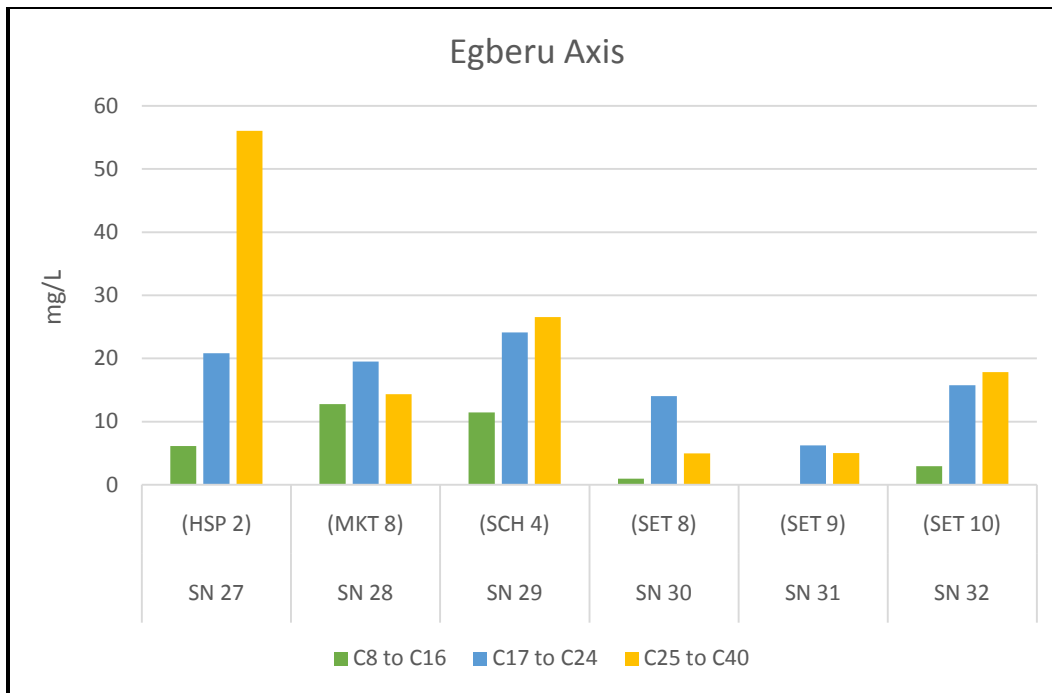
Figure 6d: Aliphatic Hydrocarbons Distribution Chart for Egberu Study Axis
