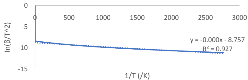
Figure 5a: KAS model-free of PET at 20°C/min
