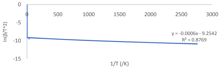
Figure 4a: KAS model free of PET at 10°C/min
