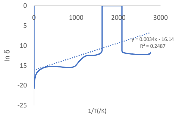
Figure 5b: CR Model-fitting of PET at 20°C /min for n = 0.25, 0.5, 0.75 and 1
