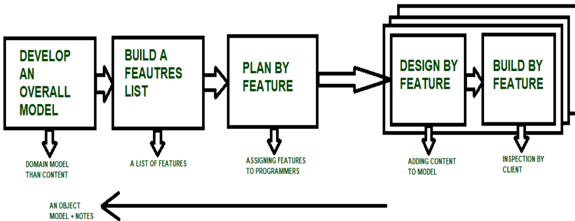
Figure 4: Feature Driven Development Model
