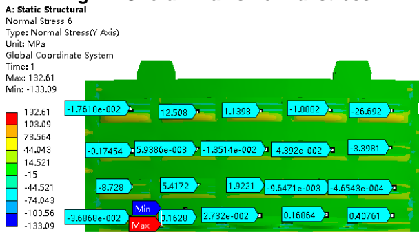
Fig.12 Overall Y-axis normal stress
