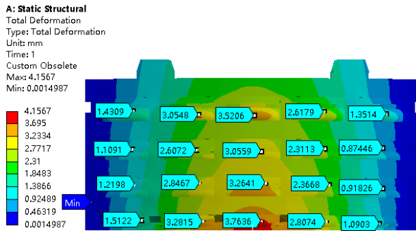
Fig.10 Global displacement contour diagram
