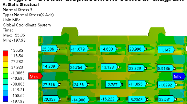
Fig.11 Overall X-axis normal stress
