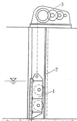
1-door leaf; 2-embedded part; 3-opening and closing equipment
