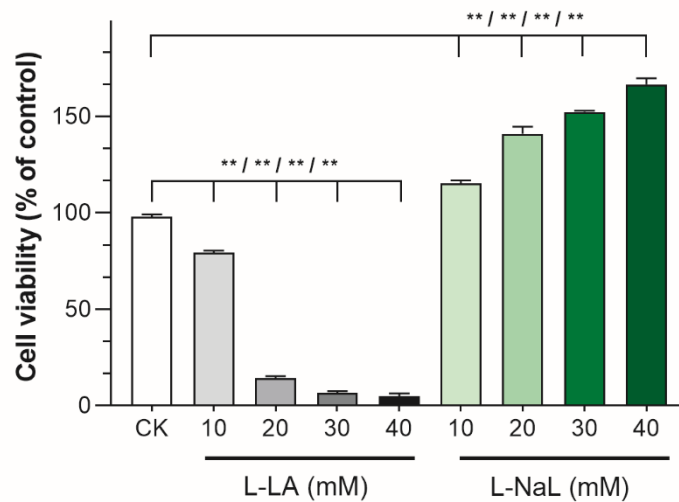
Fig. 3. Effects of NK92 cell activity treated with L-lactic acid and sodium L-lactate. CK indicates "control". " ** " indicates P < 0.01 .
