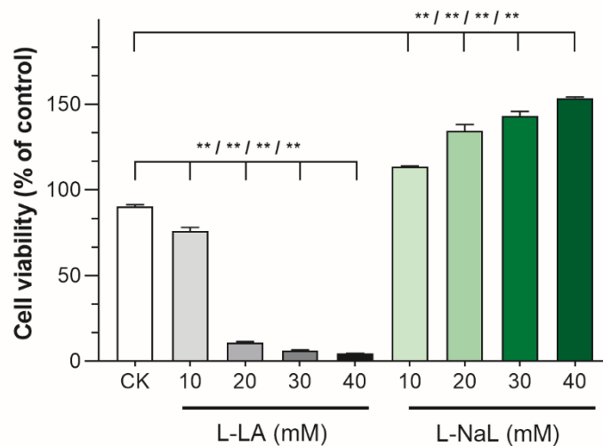
Fig. 5. Effects of NK92 cell activity treated with L-lactic acid and sodium L-lactate coexisting with 50 \mu\text{M} adenosine. CK indicates "control". " ** " indicates P < 0.01 .
