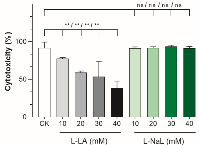
Fig. 4. Effects of NK92 cell on the killing ability of A549 cells treated with L-lactic acid and sodium L-lactate. CK indicates "control". "ns" indicates P \geq 0.05 , and " ** " indicates P < 0.01 .
