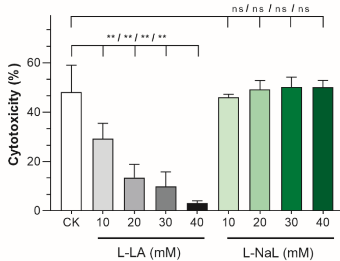
Fig. 6. Effects of NK92 cells on the killing ability of A549 cells treated with L-lactic acid and sodium L-lactate coexisting with 50 \mu M adenosine. CK indicates "control". "ns" indicates P \geq 0.05 , and " ** " indicates P < 0.01 .
