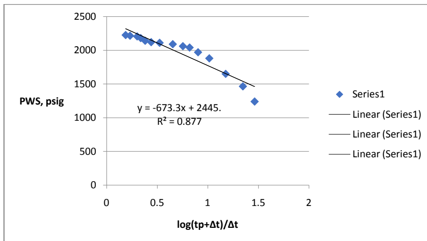
FIGURE 1: BUILD UP DATA FOR WELL 20A
