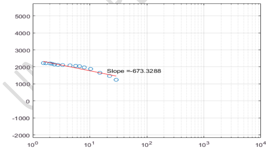
FIGURE 2: Plot of Pws Againsts (Tp+Δt)/Δt for Well 20A using matlab.
