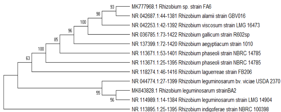
Figure 9 Neighbour joining tree based on 16S rDNA sequences showing the phylogenetic relationship of rhizobial isolates BA2 and FA6 with the analyzed sequences. (Accession numbers are mentioned within the phylogenetic tree corresponding to respective isolate)
