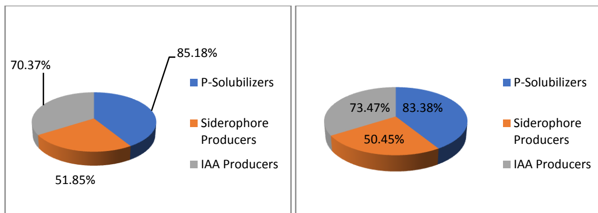
(a) (b) Figure 2: Percentage of Phosphorus solubilization, Siderophore production and IAA production by rhizobial isolates a) Himachal Pradesh b) Uttarakhand
