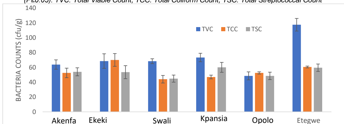
Fig. 1. A graph showing the mean count of bacteria genera from different sampling sites
