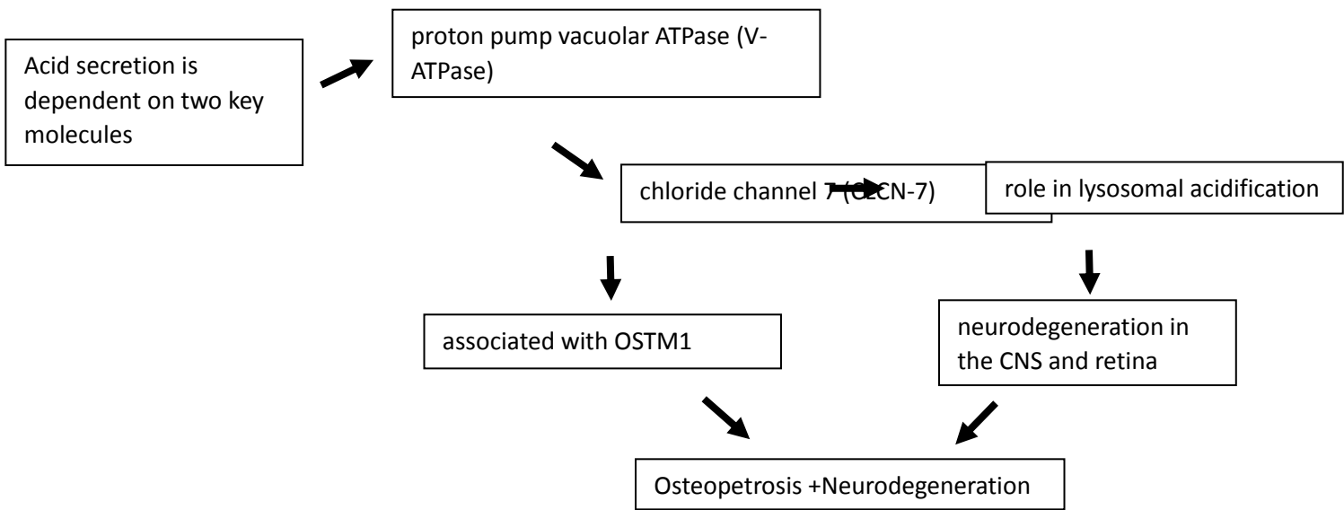
Flowchart 1: Role of V-ATPase and CLCN-7.
