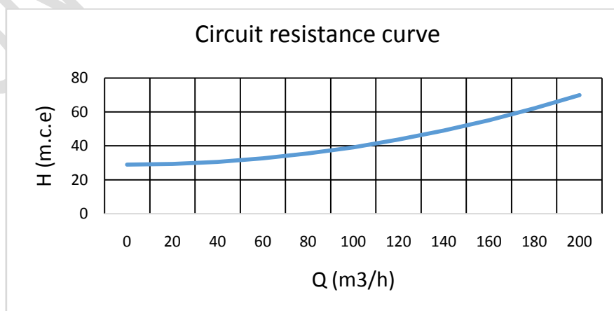
Figure 5 Circuit characteristic curve.
