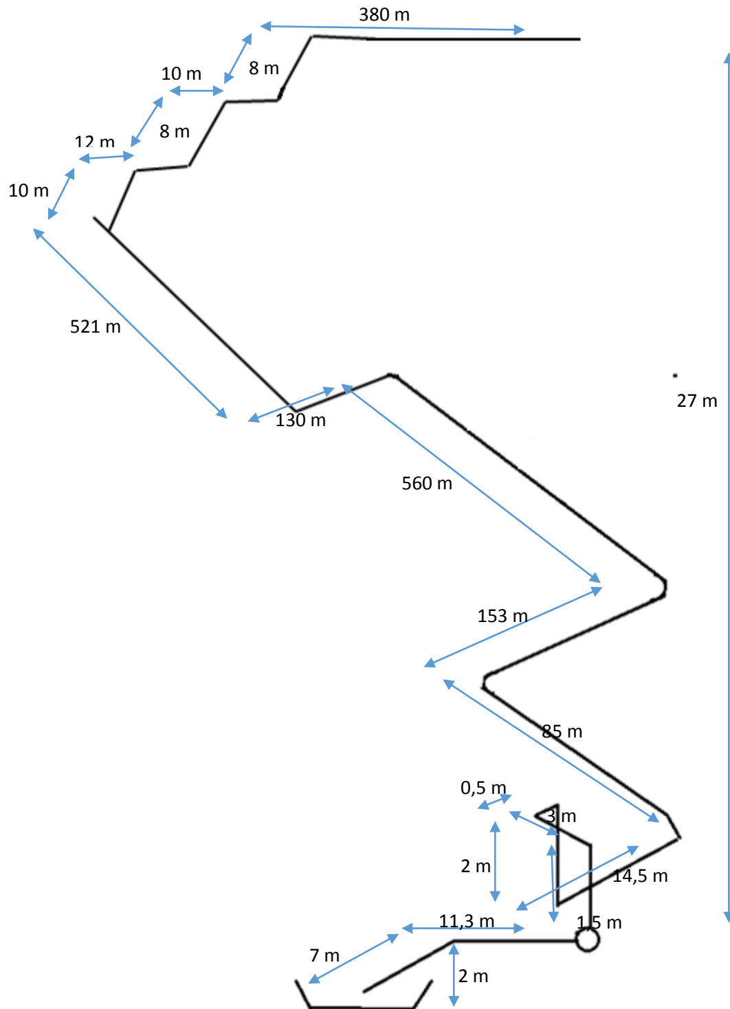
Figure 4 The pumping circuit to the end of the 3rd stage.
