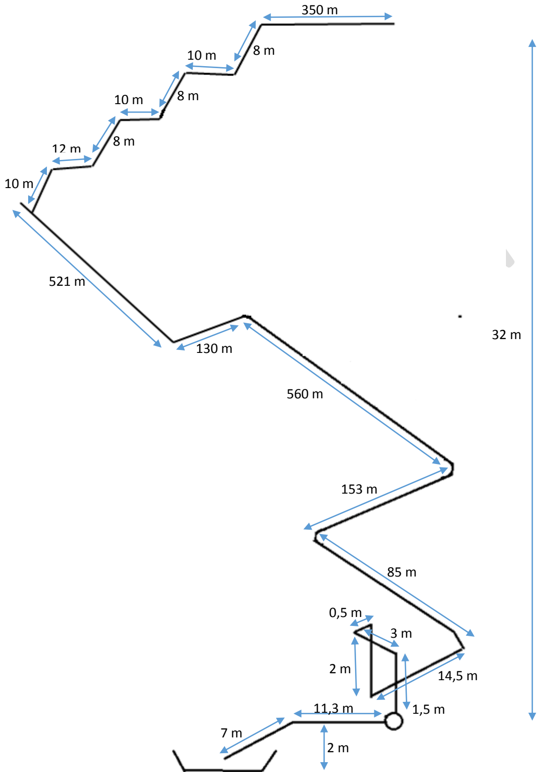
Figure 6 The pumping circuit for the 4 e stage.
