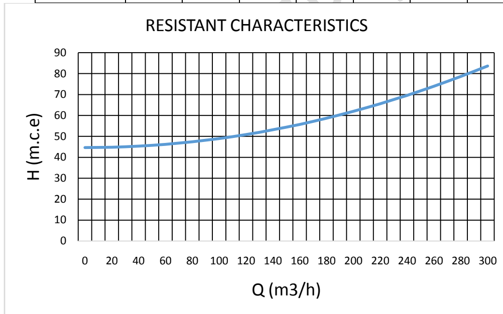
Figure 7 resistance characteristic curve.
