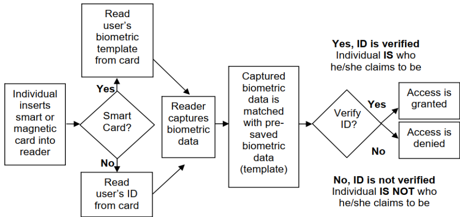
Figure 1. Biometric Authentication Algorithm
