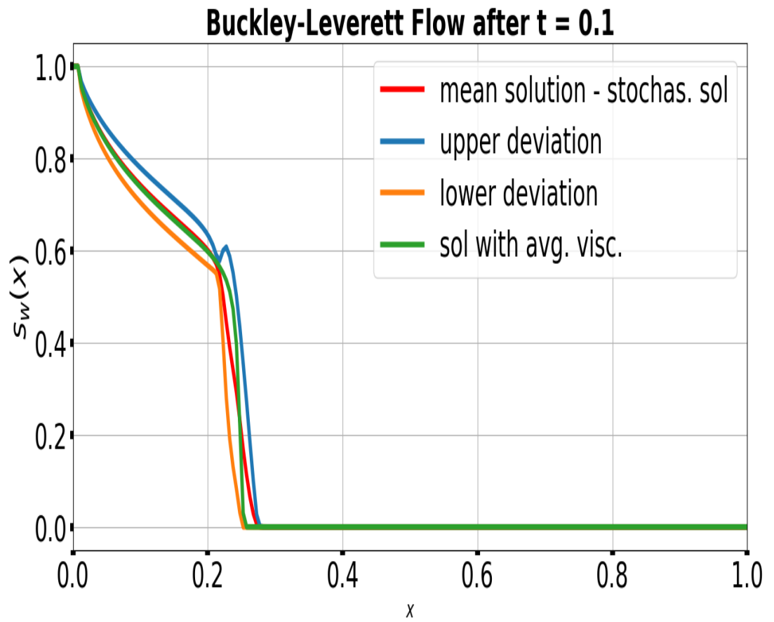
Figure 4: Stochastic solution's saturation distribution after 0.1 time units
