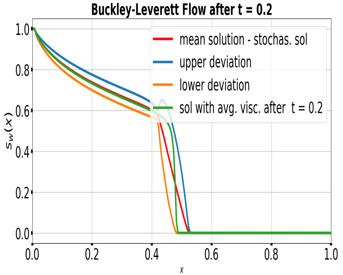
Figure 5: Stochastic solution's saturation distribution after 0.2 time units
