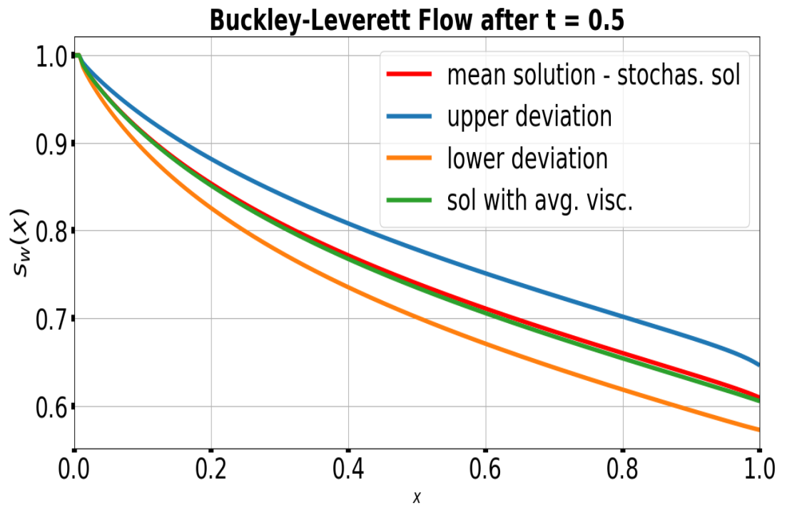
Figure 6: Stochastic solution's saturation distribution after 0.5 time units
