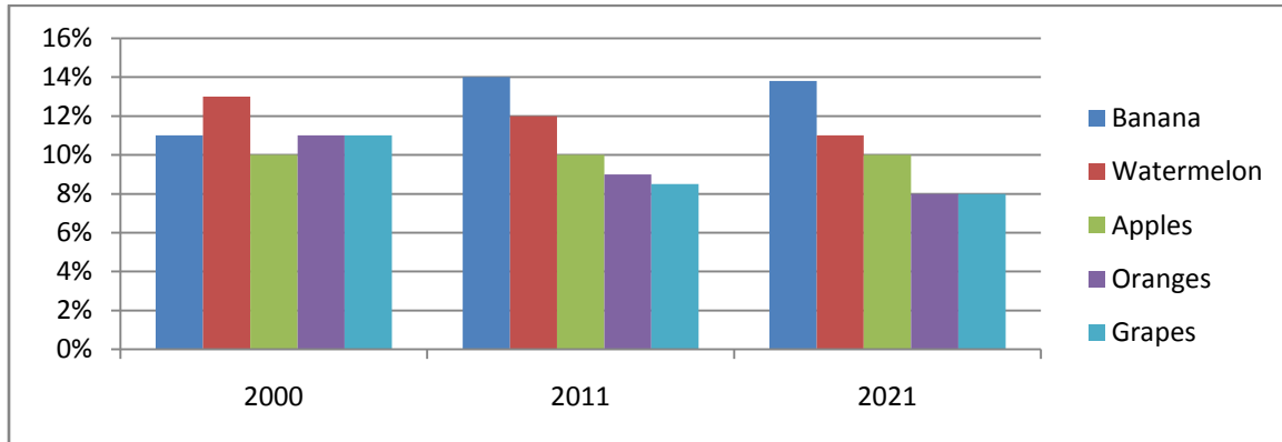
Figure 1: Top worldwide fruit production shares
