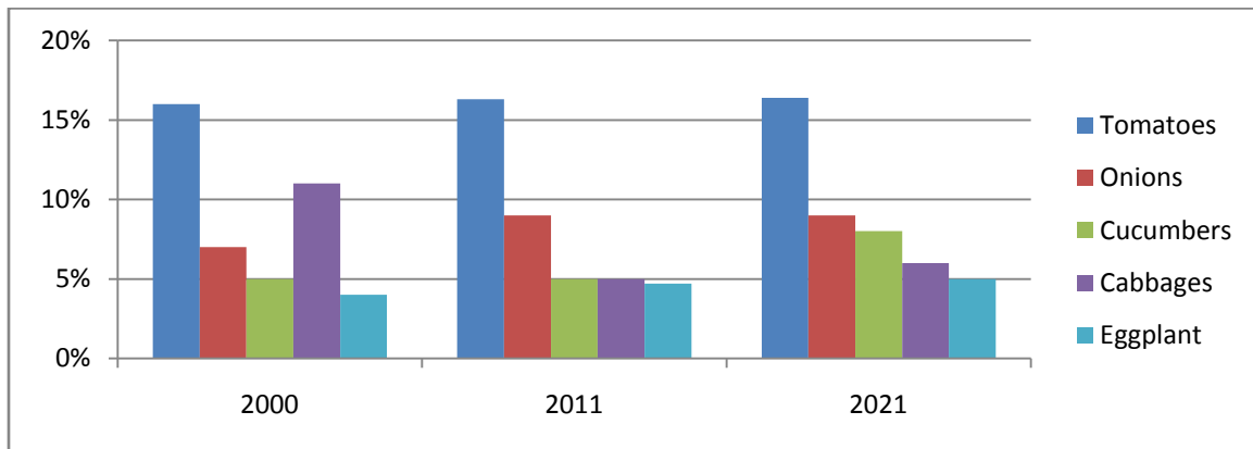
Figure 2: Top worldwide vegetables production shares
