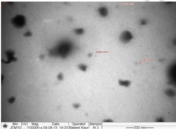
Fig 3: TEM image of Chitosan encapsulated zinc oxide nanoparticle
