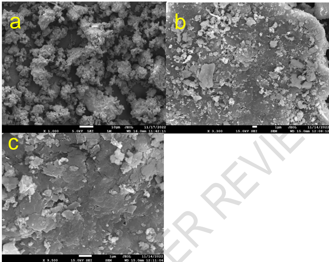
Fig 1. SEM images a) ZnO; b and c) Chitosan encapsulated Zinc Oxide nanoparticles
