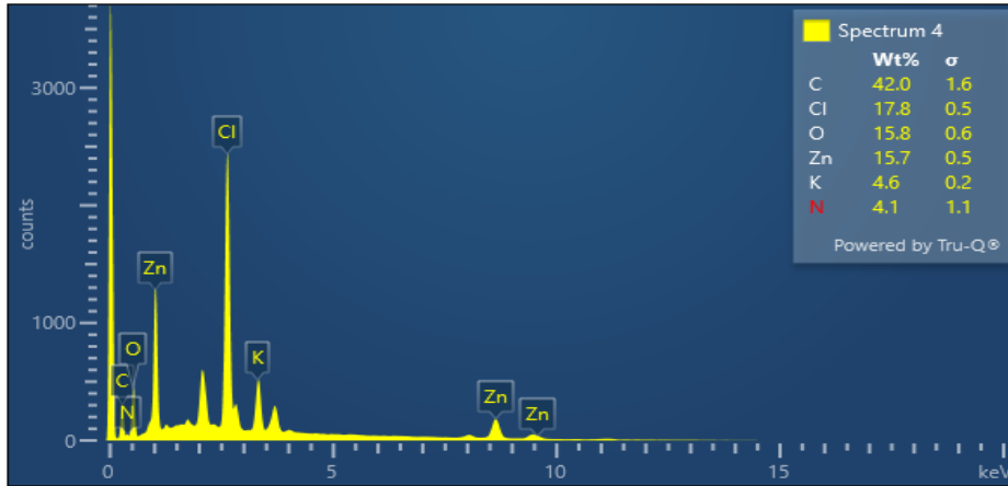
Fig 2: EDS Spectrum of Chitosan encapsulated zinc oxide nanoparticle
