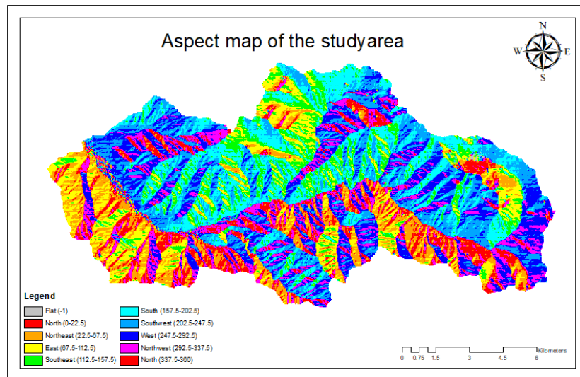
Fig. 6. Aspect map of study area
