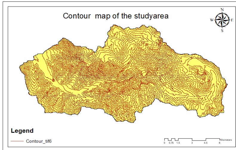
Fig. 7. Contour map of study area
