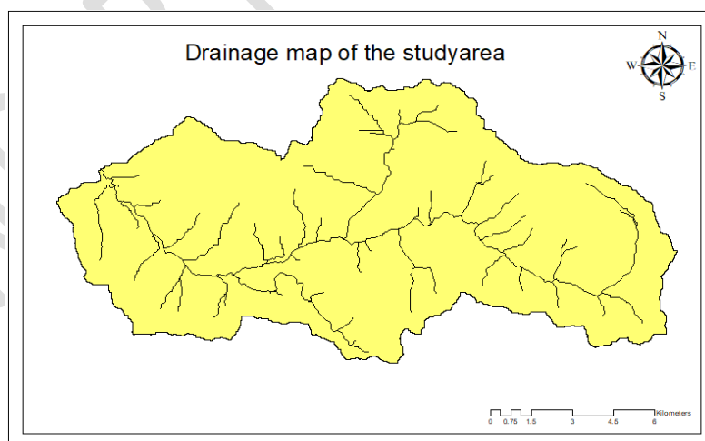
Fig. 3. Drainage map of study area
