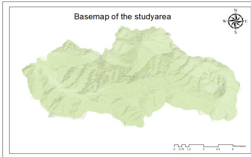
Fig. 2. Base map (toposheet) of study area
