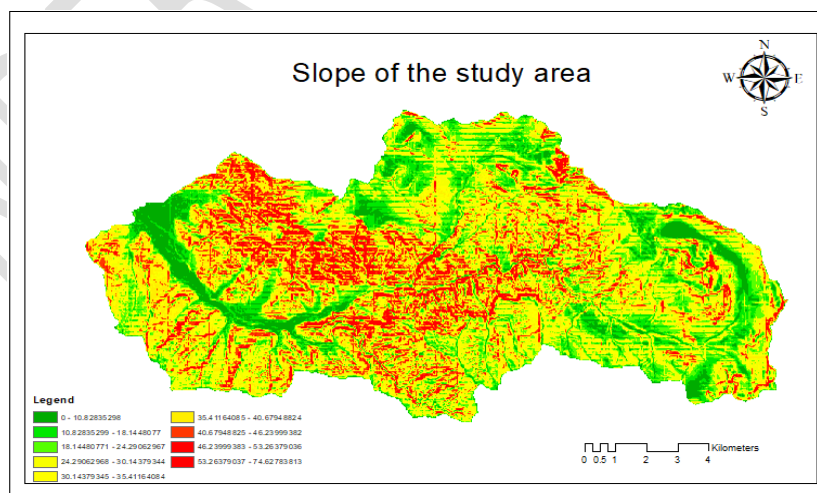
Fig. 5. Slope map of study area
